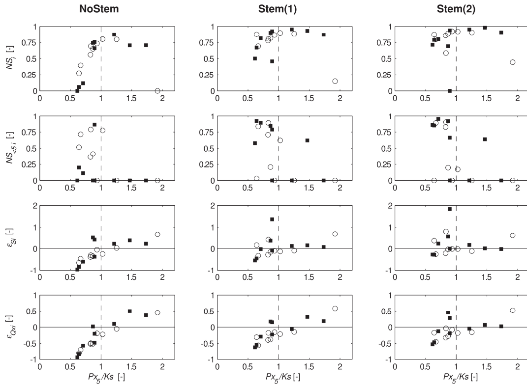
Fig. 9. Results of performance criteria for the calibration ■ and validation (○) sets for the three approaches: without stemflow NoStem and with stemflow Stem (1) and Stem (2). Px_5/Ks is the ratio between the maximal rainfall intensity for 5 min and the saturated hydraulic conductivity, NS_i and NS_{<5i} are the Nash and Sutcliffe coefficients on the whole hydrograph and on discharge lower than 5\text{ l s}^{-1} on flood recession, respectively, \varepsilon_{Si} and \varepsilon_{Qxi} the relative errors on volume and on peakflow, respectively; for graphical readability, null values are used as a substitute for negative values of NS_i and NS_{<5i} criteria.
