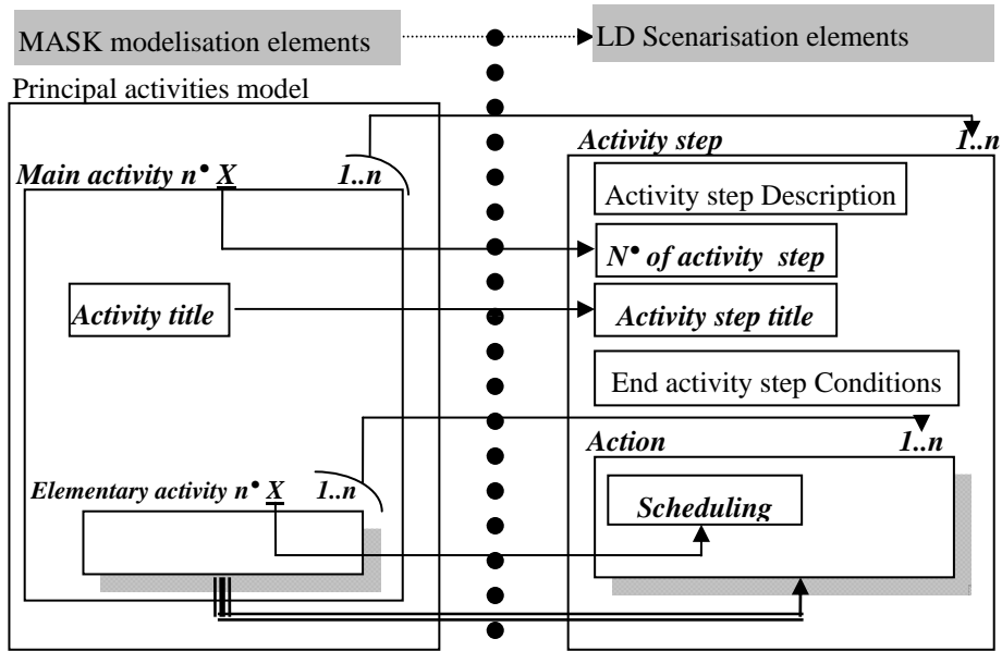
Fig. 4. Defining the different activity steps
