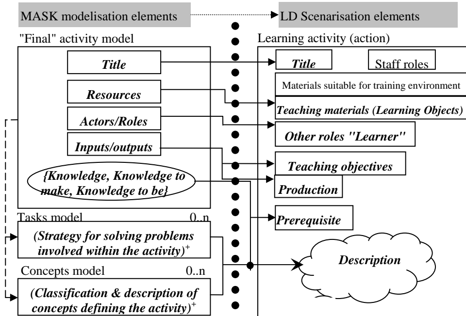
Fig. 5. Defining the details of the different activities
