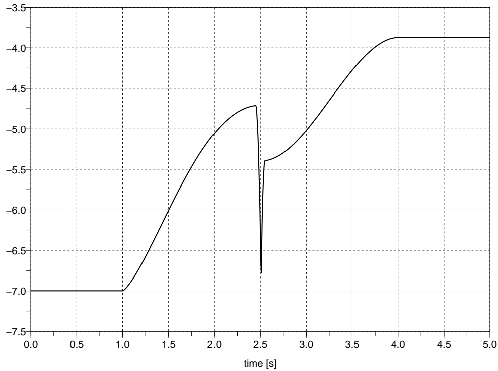
Fig. 4. Largest real part of eigenvalues of \left. \frac{\partial \mathbf{x}}{\partial \mathbf{e}} \right|_{\Gamma} (55) around the parametrization of equilibria (54)
