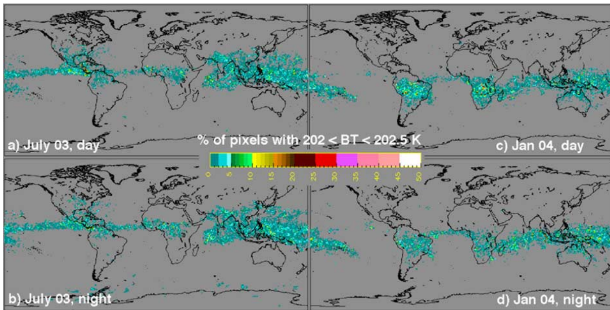
Figure 2. NAP frequencies in cloudy pixels with T_{11} between 202 and 202.5 K with NBTD between 0 and -0.5 K from MODIS/Aqua. July 2003 (a) during the day and (b) during the night. January 2004 (c) during the day and (d) during the night.
