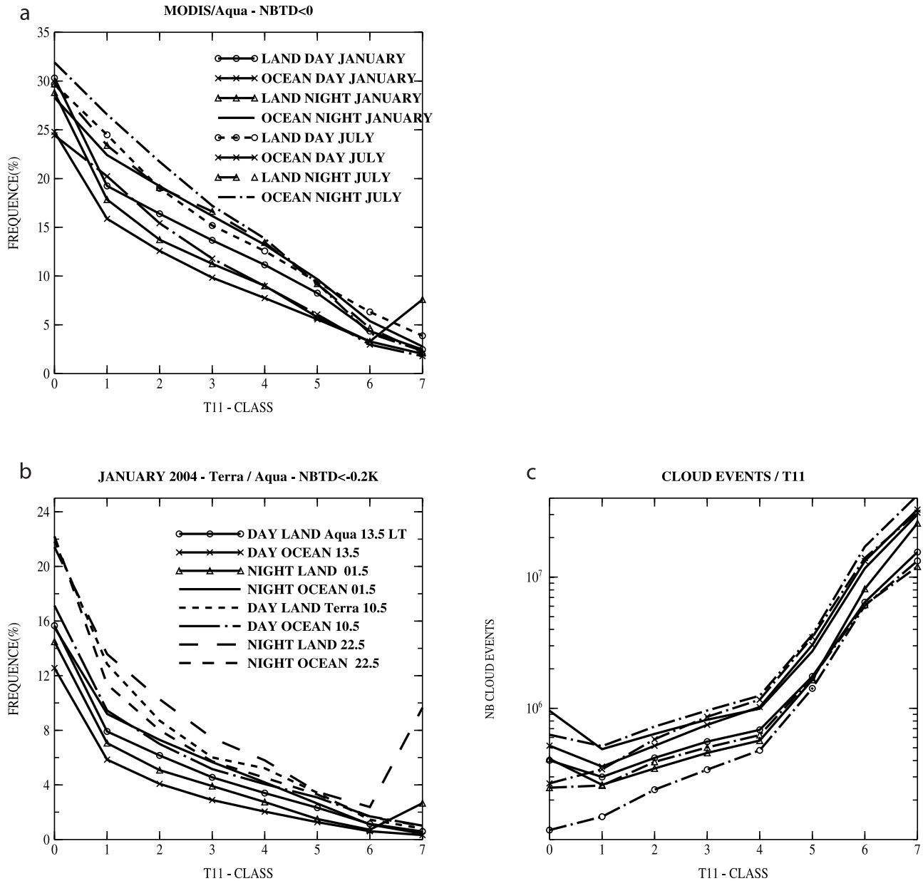
Figure 5. (a) NAP frequencies as a function of T_{11} from MODIS/Aqua in July and January. In the x axis, classes 0 to 7 correspond to T_{11} ( <195 K), (195–197.5), (197.5–200), (200–202.5), (202.5–205), (205–210), (210–220), and (220–230). (b) NAP frequencies as a function of T_{11} . Same as Figure 5a but for \text{NBTD} < -0.2 K in January only including MODIS/Aqua and Terra data. (c) Number of cloud events as a function of T_{11} in January and July from MODIS/Aqua. January (solid line) and July (dashed line).
