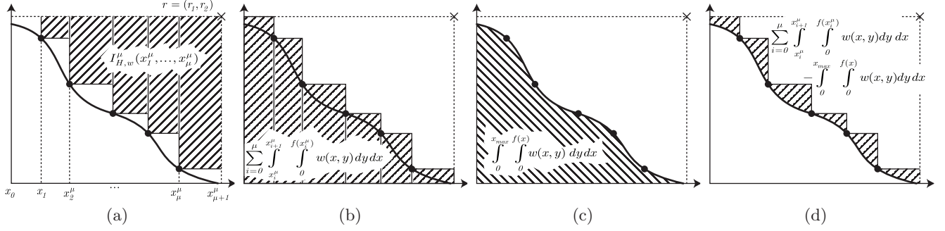
Figure 1: Illustration of the idea behind deriving the optimal density: Instead of maximizing the weighted hypervolume indicator I_{H,w}^{mu}((x_1^\mu, \dots, x_\mu^\mu)) (a), one can minimize (b) which is equivalent to minimize the integral between the attainment surface of the solution set and the front itself (c) which can be expressed with the help of the integral of f (d).
