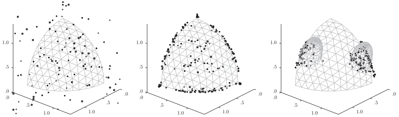
Figure 4: Pareto front approximations of five runs (depicted by different symbols) for the 3-objective DTLZ2 test problem using NSGA-II (left), IBEA (middle), and HypE with two preference points displayed as ellipsoids (right).
