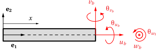
FIGURE 8: Notations for a straight beam in its local reference frame
