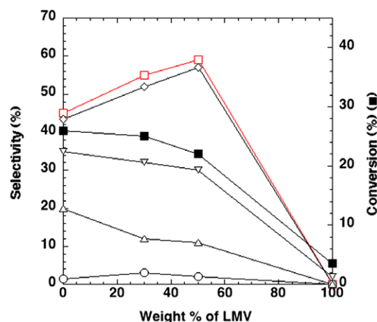
Fig. 2. Variation of the conversion of isobutane (■) and of the selectivity in MAA + MA (□), MAA (◆), MA (○), AcA (△), and CO x (▽) as a function of the wt.% of LMV1 (LMV with 6 m 2 g -1 ) in the CsTeV-LMV phase mixtures. The reaction was run at 360 °C; feedstock composition: \text{O}_2/\text{C}_4\text{H}_{10}/\text{H}_2\text{O}/\text{N}_2 = 10/10/10/70 ; total flow = 30 mL min -1 .
