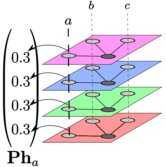
Fig. 3. Long-term system architecture before learning: in this example, the user's computer is linked to three target hosts a , b and c . There are four planes available to catch the distribution of the categories. The probabilities to visit a host are uniform for each plane. For instance, the probability to visit a is 1/3 on all of the four planes.
