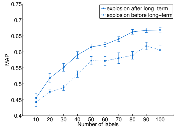
Fig. 11. MAP for the category explosion-fire before and after learning. With the long-term optimization, the gain is about 8% and the speed-up is about 60 labels.
