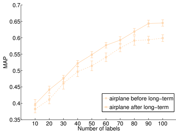
Fig. 9. MAP for the category airplane before and after learning. With the long-term optimization, the gain is about 5% and the speed-up is about 30 labels.
