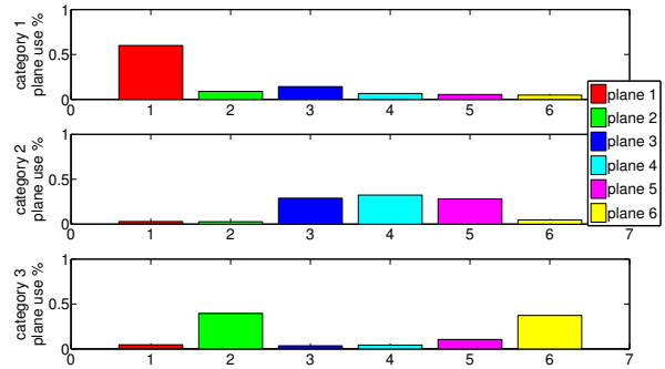
Fig. 7. Percentage of markers that were used for each category. Markers have been at most used for the category towards which destination they routed. For example, for the third category, the most used markers where the second and the sixth, which are leading to the host containing the third category as seen on Fig. 5
