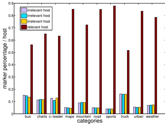
Fig. 2. Results of the routing learning system : final probability score P_i of an agent to move to each host at the end of a retrieval session depending on the category being searched. In our experiment, fourth host of the four destinations available contained the relevant category. At the end of a session, its probability P_4 of being visited is the highest.
