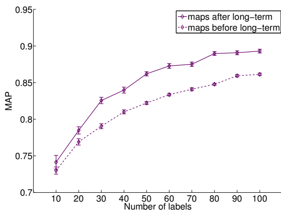
Fig. 10. MAP for the category maps before and after learning. With the long-term optimization, the gain is 5% and the speed-up is about 50 labels.
