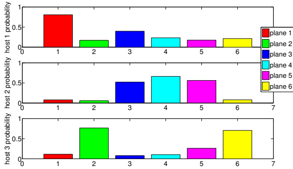
Fig. 5. Relative values of each marker on the three hosts. Each of the six planes has been specialized for one host. For example, the first plane has a higher probability to lead to the first host, while the second plane has a higher probability to lead to the third host.
