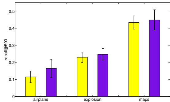
Fig. 8. Recall for each category for 500 images retrieved, compared to a classical CBIR system. The distributed system performs a little better on more difficult categories as airplane or explosion-fire .
