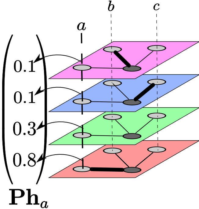
Fig. 4. Example of the long-term system after learning: Some of the planes have specialized into one category. For instance, the fourth plane has specialized to the category contained on host a and therefore its probability of being visited using this plane is 0.8.
