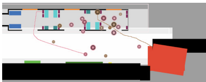
Fig. 2. Screenshot of the first version of SimTRAP showing passengers leaving and entering the train
