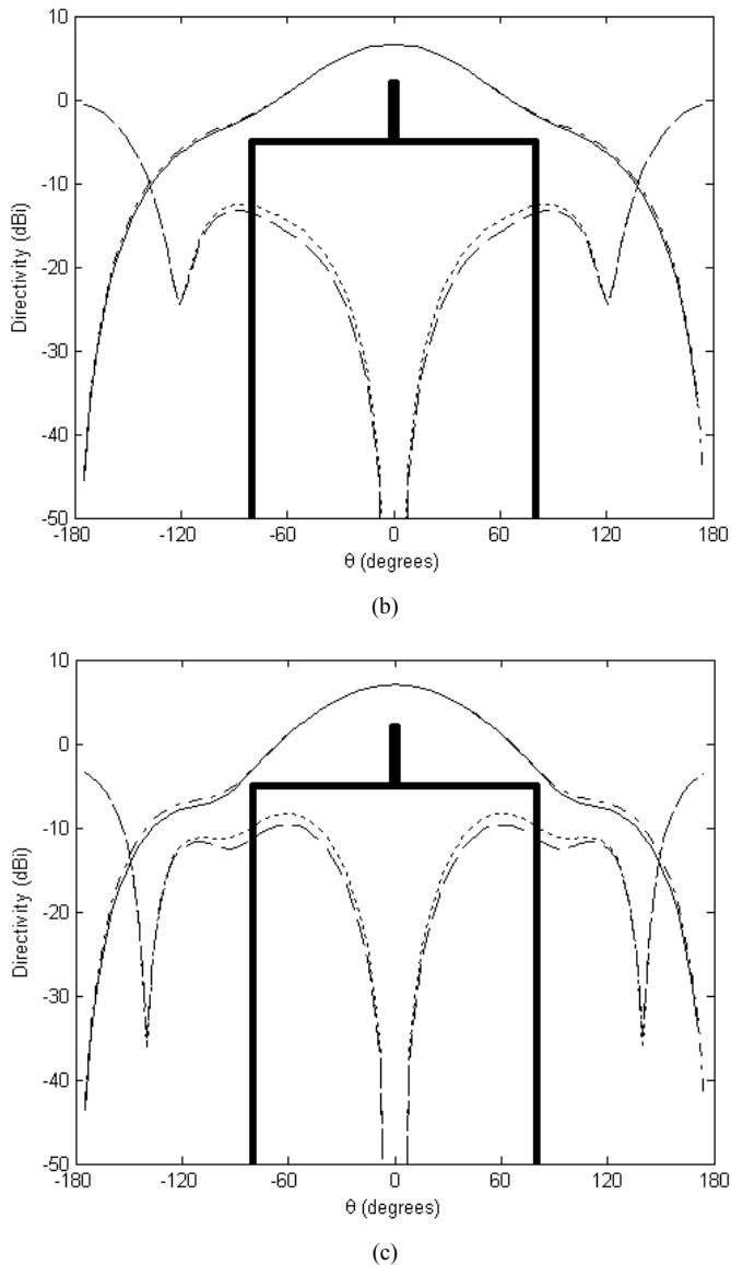
Fig. 4 Simulated radiation patterns at: (a) 1.189GHz, (b) 1.280GHz and (c) 1.575GHz. \phi = 0^\circ : (—) RH-CP, (- - -) LH-CP; \phi = 45^\circ : (— —) RH-CP, (— —) LH-CP; (█) Minimum required RH-CP
