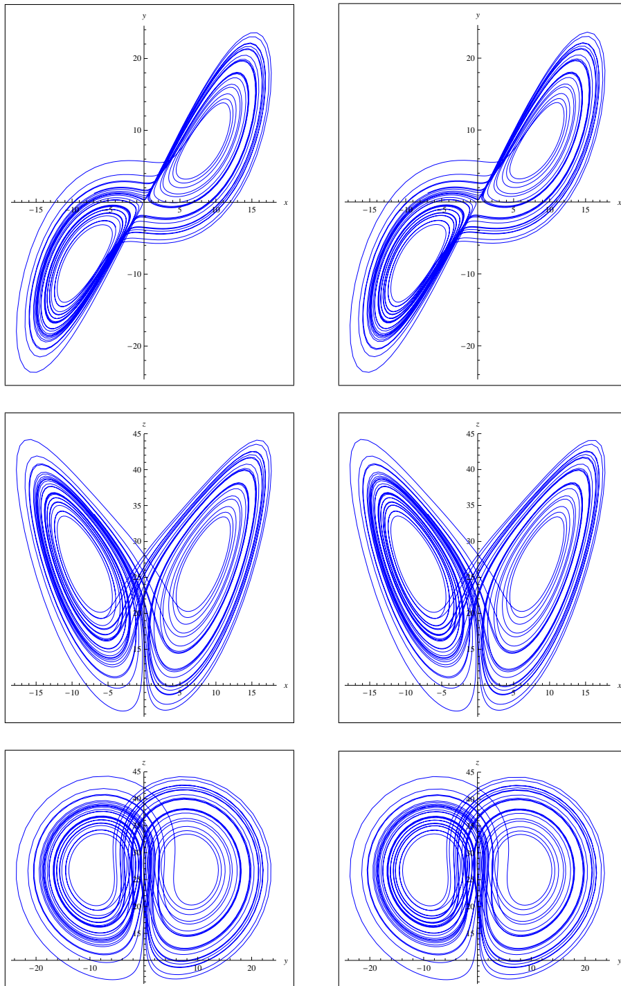
Figure 6: Chaotic attractors for the chaotic Lorenz system (19), comparison between Multi-step DTM (Left) and RK4 method (Right).
