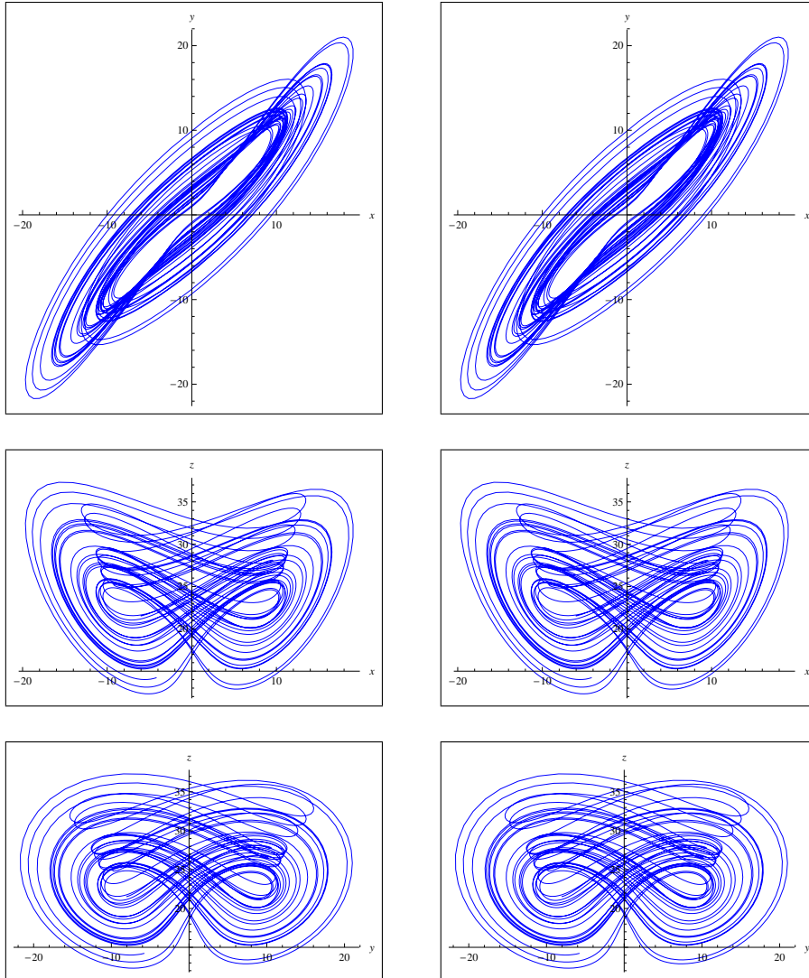
Figure 3: Chaotic attractors for the chaotic Chen system (16), when (a, b, c) = (35, 3, 28) , comparison between Multi-step DTM (Left) and RK4 method (Right).
