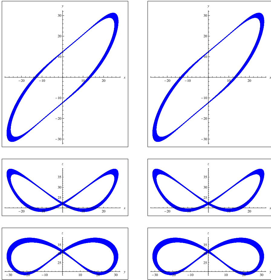
Figure 4: Chaotic attractors for the chaotic Chen system (16), when (a, b, c) = (35, 12, 28) , comparison between Multi-step DTM (Left) and RK4 method (Right).
