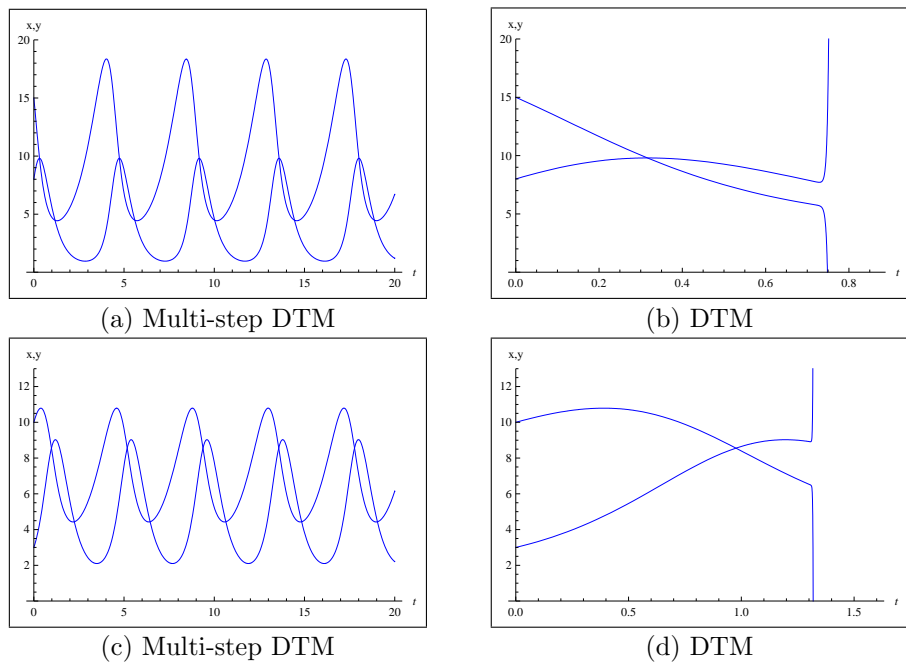
Figure 2: Time series for Lotka-Volterra system (10), comparison between Multi-step DTM and DTM. Obviously the DTM solution diverges for t > 0.75 in (b) and t > 1.35 in (d).
