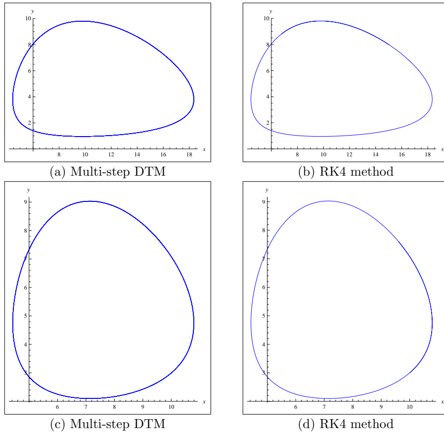
Figure 1: Phase plane trajectories for Lotka-Volterra system (10), comparison between Multi-step DTM and RK4 method.
