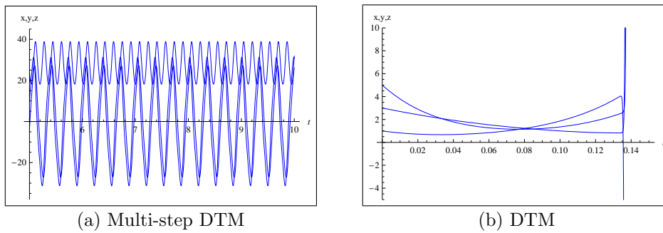
Figure 5: Time series for the chaotic Chen system (16), comparison between Multi-step DTM and DTM. Obviously the DTM solution diverges for t > 0.135 .
