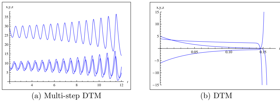
Figure 7: Time series for the chaotic Lorenz system (19), comparison between Multi-step DTM and DTM. Obviously the DTM solution diverges for t > 0.15 .
