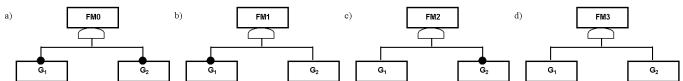
Figure 4. Fault trees for failure modes
