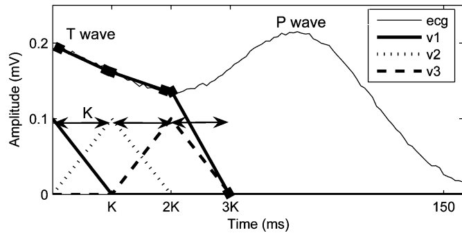
Fig. 2. Example of a real T wave modeled as a decreasing piecewise linear function based on three functions v_l ( M_{P-3} ). The piecewise function corresponds to the estimated T wave by the proposed method using the vectors v_1 , v_2 , and v_3 in a real case.
