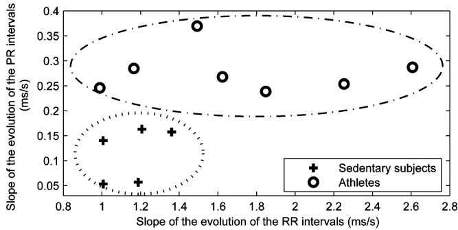
Fig. 7. Relationship between the slope of the evolutions of the PR and RR intervals for the 12 subjects. The two groups can be clustered according the PR slopes.
