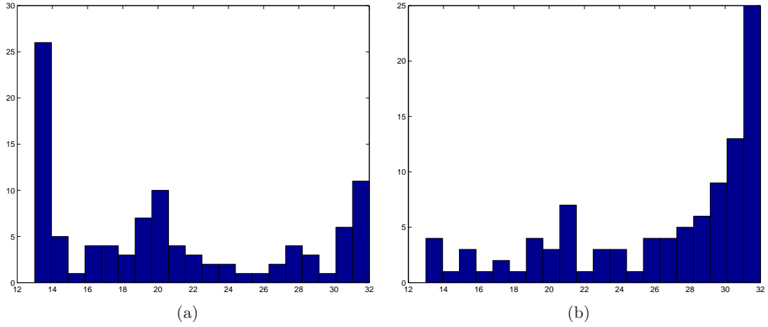
Figure 2: Selection of the frequency cut-off over M = 100 replications of the simulations (with m_0 = 32 ): (a) Histogram of the selected value for N^* , (b) Histogram of the selected value for \tilde{N} .
