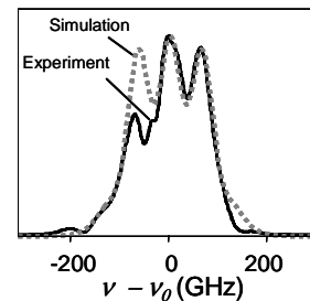
Fig. 9. Output spectrum for the 1.15-m long AsSe chalcogenide fiber for an input average power of 1 mW, dashed-line: corresponding numerical simulation.
