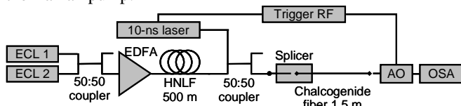
Fig. 12. Experimental set-up for Raman characterization.
