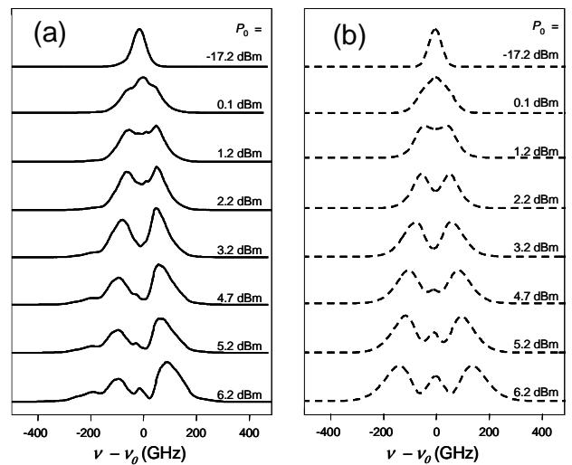
Fig. 8. (a) Experimental results: output spectra for the 1.45-m long GeSbS_1 chalcogenide fiber as a function of input power (b) Numerical simulations corresponding to results of Fig. a.
