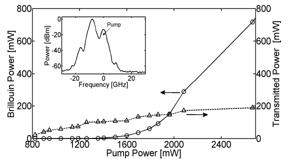
Fig. 11. Inset: Experimental Brillouin spectrum recorded at port #3 of the circulator for the 2-m long GeSbS_2 chalcogenide fiber. Backscattered and transmitted powers as a function of the input power Chalcogenide fiber.
