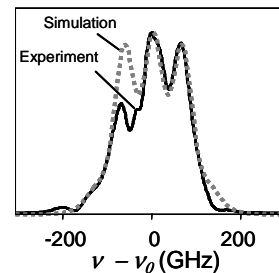
Fig. 9. Output spectrum for the 1.15-m long AsSe chalcogenide fiber for an input average power of 1 mW, dashed-line: corresponding numerical simulation.
