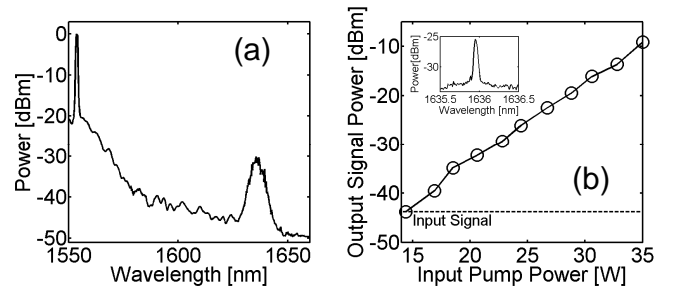
Fig. 13. (a) Spontaneous Raman scattering at the output of the GeSbS 2 chalcogenide fiber for an input pump power of 80 W. (b) Output signal power as a function of input pump power for the chalcogenide fiber. Inset: Output amplified signal spectrum for a pump power of 24.5 W.
