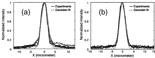
Fig. 2. Experimental traces (solid line) of the intensity distribution in the near field of the GeSbS_1 fiber (a) and the AsSe fiber (b). Squares represent a Gaussian fit distribution.
