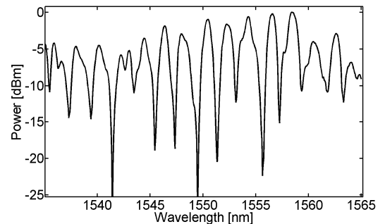
Fig. 6. Interference fringes at the chalcogenide GeSbS_1 fiber output.
