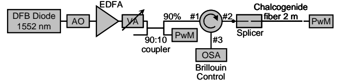
Fig. 10. Experimental set-up for Brillouin Characterization.
