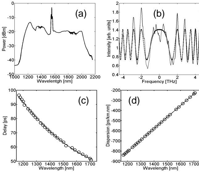
Fig. 4. (a) Supercontinuum generated at the output of the HNLf fiber (b) Interference fringes at the coupler output (c) Delay vs wavelength, experimental values for the GeSbS_2 fiber (circles), polynomial fit (solid line) (d) Dispersion vs wavelength, experimental values (circles), linear fit (solid line).
