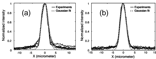
Fig. 2. Experimental traces (solid line) of the intensity distribution in the near field of the GeSbS_1 fiber (a) and the AsSe fiber (b). Squares represent a Gaussian fit distribution.
