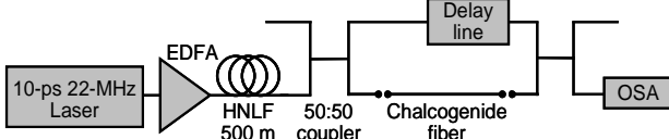
Fig. 3. Experimental set-up for chromatic dispersion characterization.
