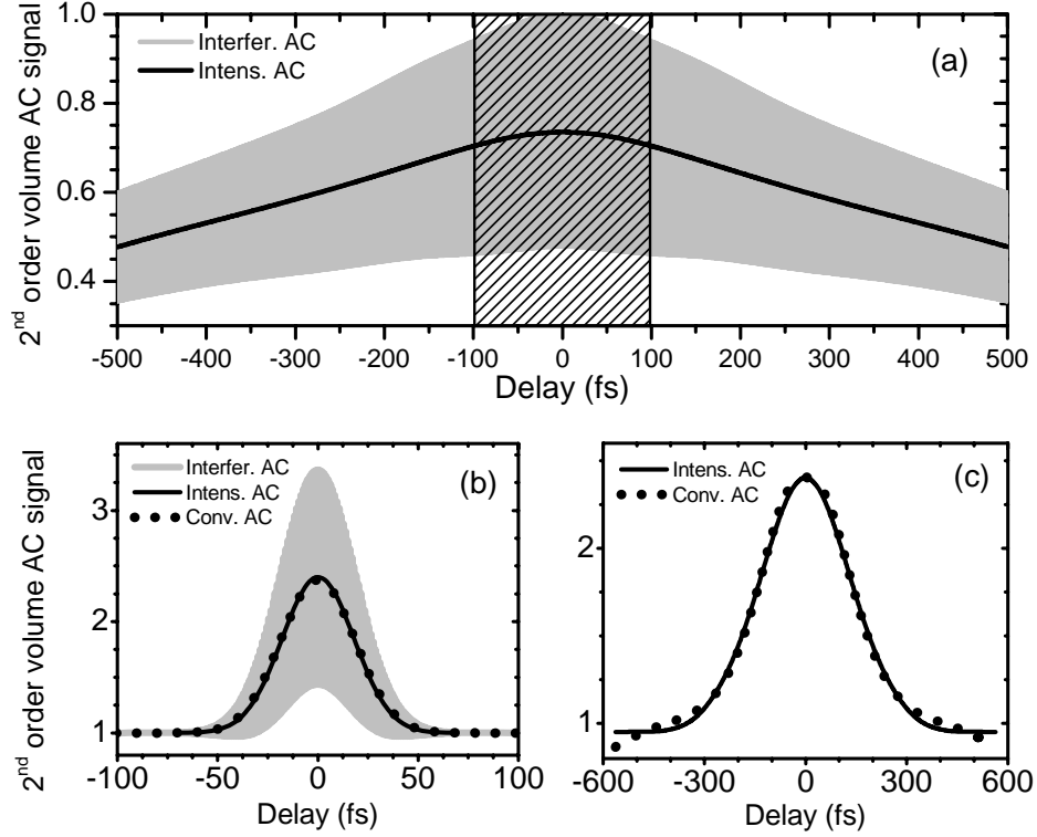
FIGURE 4. Model calculations of the 2 nd order volume interferometric (grey shaded areas) and intensity (black solid lines) AC traces for a a) CW laser, b) 30 fs, and c) 200 fs pulses. Black dots: Conventional 2 nd order intensity volume AC traces. The 200 fs shadowed area in graph 3a depicts the area of negligible (< 5 %) deviation of the AC signal due to spatial displacement for the tight focusing conditions considered here (see text for details).
