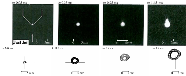
Fig. 20. Kernel growth, comparison between experimental [25] and LES results. Spark location: z = 30 d_j .
