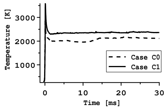
Fig. 32. Ignition case C0: a) flame topology (black line: stoichiometry, gray line: lean flammability limit); b) temporal evolution of the maximum flame temperature for cases C0 and C1.
