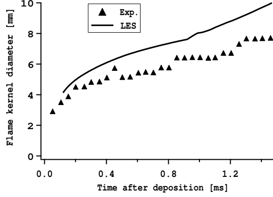
Fig. 20. Kernel growth, comparison between experimental [25] and LES results. Spark location: z = 30 d_j .
