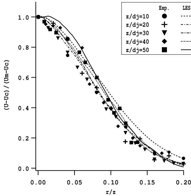
Fig. 11. Radial distribution of the mean axial velocity ( U ) scaled by the mean axial velocity on the axis ( U_m ), comparison of the experimental data of Ahmed et al. [25] (symbols) and LES results (lines). Air jet, injection velocity: U_j = 21 \text{ m/s} and co-flow velocity: U_c = 0.1 \text{ m/s} .
