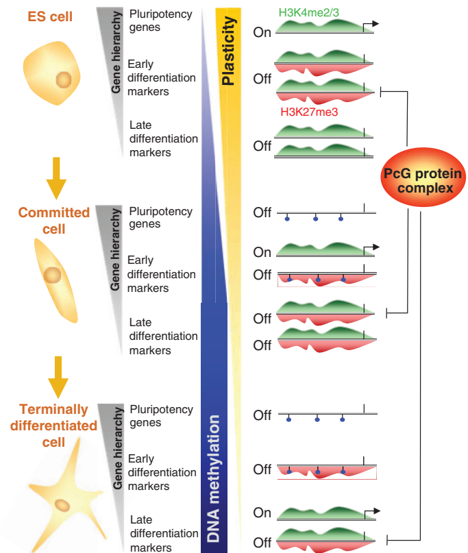
Fig. 3. PcG protein complexes dynamically regulate the gene hierarchy during cell fate choice. In embryonic stem (ES) cells, early differentiation marker genes are repressed by PcG protein complexes (indicated by T-bars), which ensures the stable maintenance of ES cell identity. The majority of PcG protein target genes are also methylated at H3K4, an active mark (green domain), in addition to H3K27, a repressive mark (red domain), and are therefore in a bivalent state. Late differentiation markers can be methylated at H3K4, but are not expressed. Upon cell fate commitment, early differentiation markers involved in the appropriate lineage become activated and lose the repressive H3K27me 3 mark, while other ES cell-specific bivalent genes that are repressed during early lineage commitment maintain H3K27 methylation but lose H3K4 methylation and become de novo DNA methylated (blue circles). Pluripotency genes become stably repressed and gain DNA methylation. Note that the majority of DNA methylation occurs during early lineage commitment, whereas DNA methylation is less dynamic during the transition to a terminally differentiated state. By contrast, the PcG protein machinery moves down the gene differentiation hierarchy to repress late differentiation markers upon lineage commitment (indicated by repressive linkers). Importantly, these genes become methylated de novo at H3K27, resulting in the formation of new bivalent domains. Upon terminal differentiation, some of these late differentiation markers become activated (resulting in a concomitant loss of H3K27me 3 ), while other genes that became new PcG protein targets during cell commitment remain in a repressed state. Note that the total number of bivalent domains does not change significantly during differentiation.
