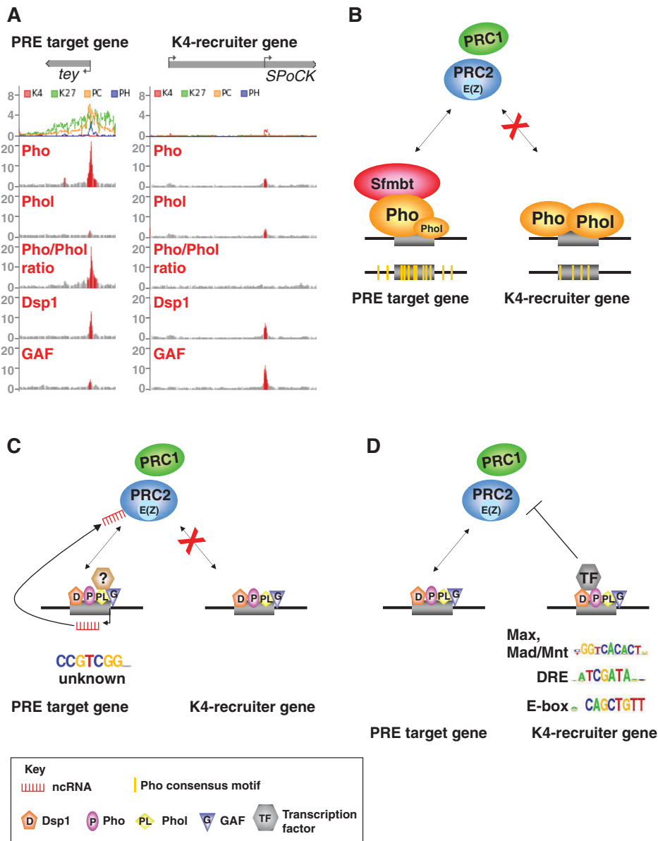
Fig. 2. Models of PcG protein recruitment to PREs. (A) Comparative analysis of the chromatin state of the teyrha-meyrha ( tey ) gene, a PRE target gene, versus the Secretory Pathway Calcium ATPase ( SPoCK ) gene, which is not bound by PcG protein complexes. Top tracks show ChIP-on-chip profiles of the PcG proteins Polycomb (Pc) and Polyhomeotic (Ph) and of the histone marks H3K27me3 (K27) and H3K4me3 (K4) in Drosophila embryos. Lower tracks show ChIP-on-chip profiles of the indicated DNA-binding proteins. The binding ratio between the homologous proteins Pho and Phol is high at PcG response elements (PREs), but low at K4-recruiter genes. (B) A high Pho/Phol binding ratio might be essential for targeting the PhoRC complex to PREs, which in turn might anchor PRC2 and PRC1 to PREs. Note that Pho sequence motif distribution is denser and less tightly localized at PREs compared with K4-recruiter loci. (C) PcG protein complex recruitment to PREs might be mediated by unknown DNA-binding proteins (indicated by a question mark) that are absent from K4-recruiter loci and act together with previously identified PcG protein recruiters such as Dsp1 (D), Pho (P), Phol (PL) or GAF (G). In addition, non-coding RNAs (ncRNAs) might help to recruit PcG protein complexes. (D) Transcription factors (TF) bound at K4-recruiter sites might block the recruitment of PcG protein complexes. Sequence motifs that are overrepresented in either PREs or K4-recruiter sites are shown below C and D.
