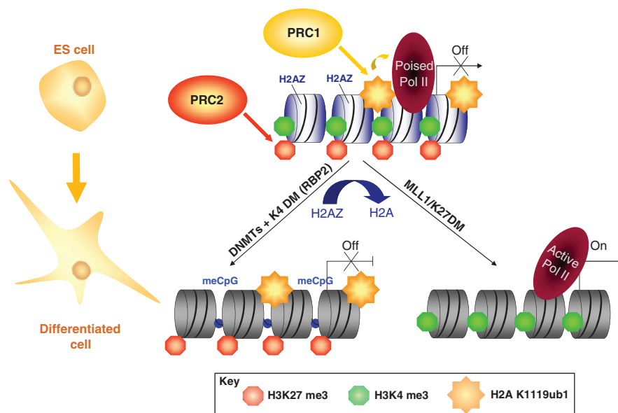
Fig. 4. Resolution of bivalent chromatin domains during ES cell differentiation. Key developmental regulators are marked bivalently by the histone marks H3K27me3 and H3K4me3 in ES cells. Many of these bivalently marked genes are bound by a non-processive form of RNA polymerase II (poised pol II). PRC1-mediated ubiquitylation of histone H2A on lysine 119 (H2AK119ub1) is essential to keep RNA pol II in a poised configuration. In addition, the histone variant H2AZ marks many silent key developmental regulators and might protect these genes from DNA methylation and stable silencing. Upon differentiation, activated bivalent genes lose the repressive H3K27me3 mark, and H2AZ is redistributed to a different set of genes that is highly active. MLL1 has been shown to be required for the resolution of specific bivalent domains, possibly by recruiting H3K27-specific demethylases (K27DM). By contrast, bivalent genes that remain inactive in differentiated cells lose the active H3K4me3 mark owing to the activity of K4-specific histone demethylases (K4DM), such as RBP2. The replacement of H2AZ by H2A might contribute to CpG island methylation (meCpG, blue circles), which leads to stable gene silencing.
