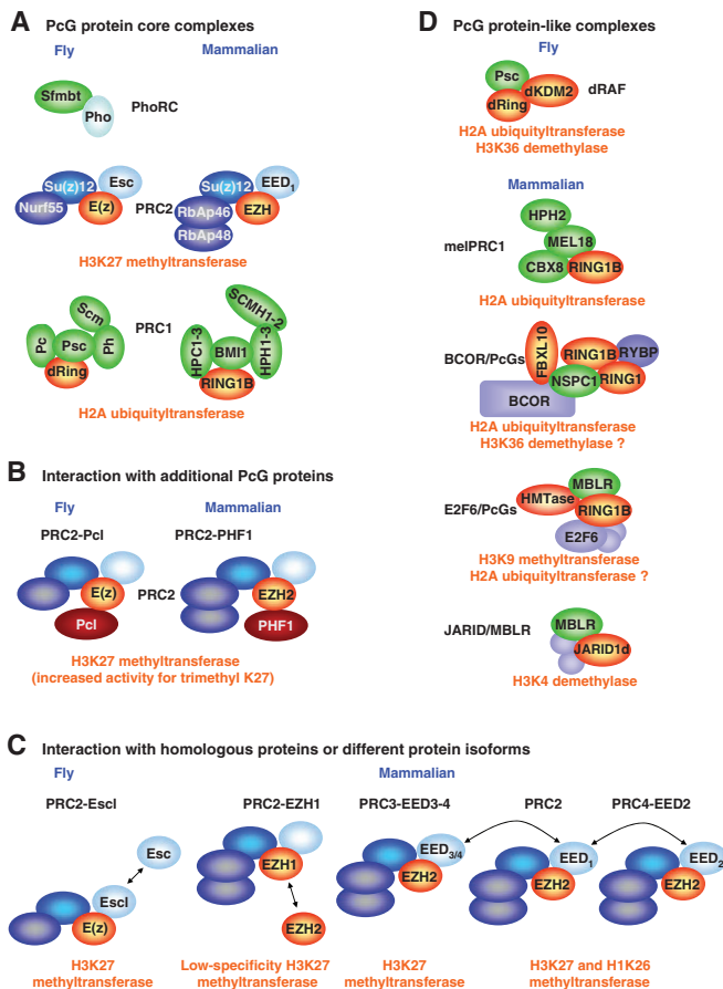
Fig. 1. PcG protein complex diversity. (A) The three principal Polycomb group (PcG) complexes in Drosophila and mammals. (B-D) Additional PcG protein complex diversity is achieved (B) by the interaction with additional PcG proteins, (C) by the incorporation of homologous proteins or different protein isoforms, or (D) by PcG protein-like complexes that include only some of the PRC1 core components in combination with other chromatin regulators. The major enzymatic components of each complex are shown in red, and their known biochemical activities are indicated below each complex.
