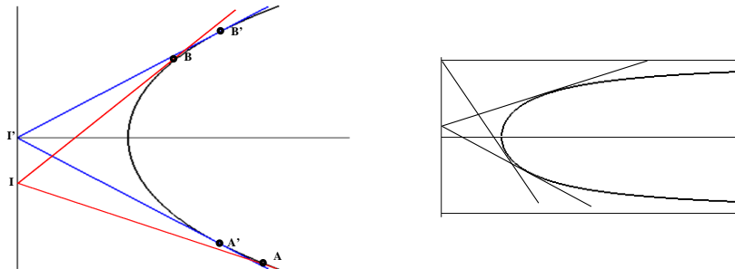
Figure 1: Catenaries, n \geq 2 and n \geq 3
