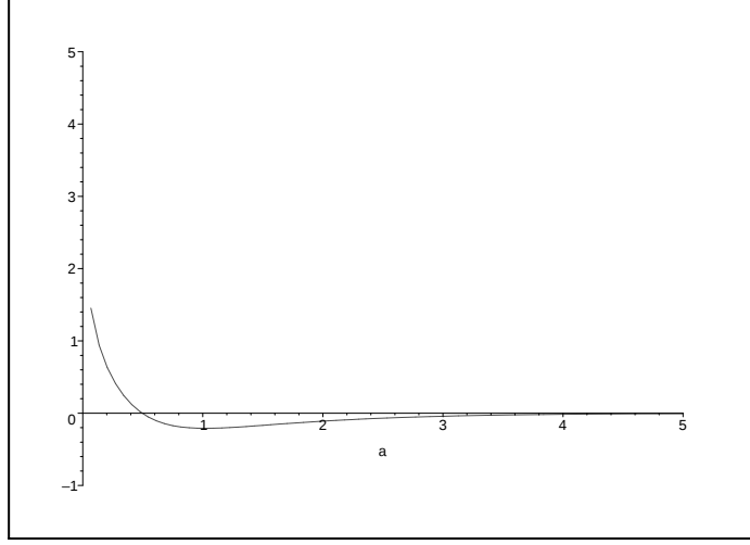
Figure 4: Graph of E_0(a)
