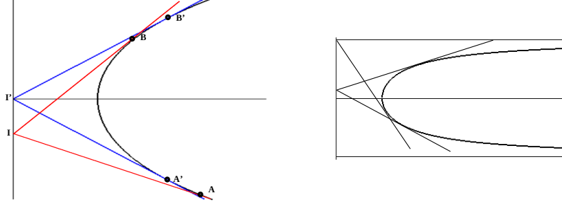
Figure 1: Catenaries, n \geq 2 and n \geq 3
