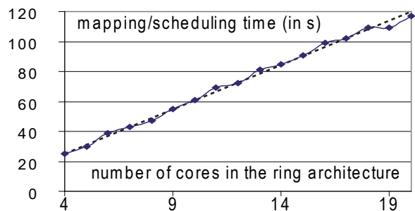
Figure 13. mapping/scheduling time of an LTE algorithm on ring architectures with increasing number of cores
