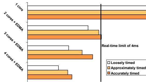
Fig. 18. Timings of the RACH-PD algorithm schedule on target architectures
