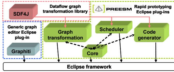
Fig. 1. An Eclipse-based Rapid Prototyping Framework
