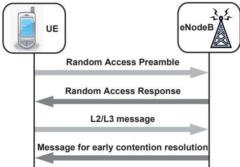
Fig. 14. Random access procedure
