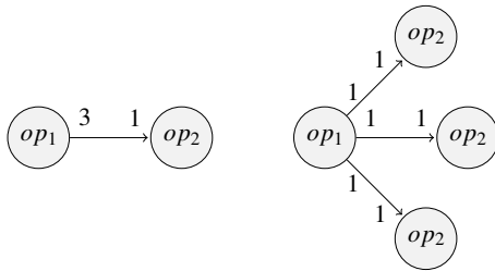
Fig. 7. A SDF graph and its HSDF transformation
