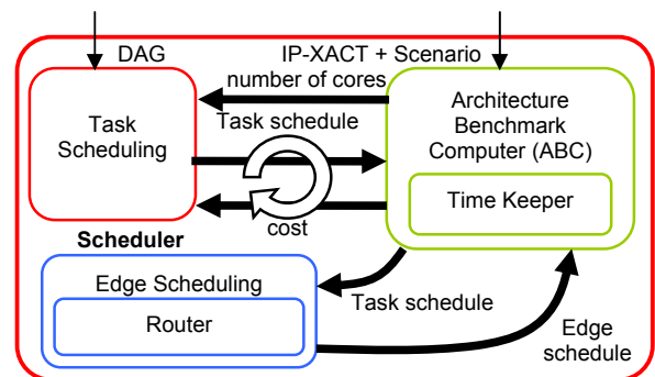
Fig. 9. Scheduler module structure
