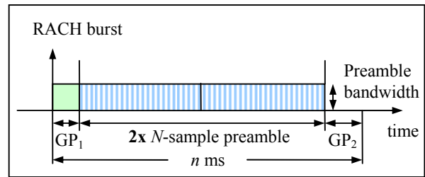
Fig. 15. The random access slot structure
