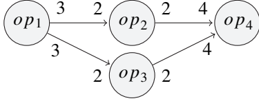
Fig. 6. A SDF graph
