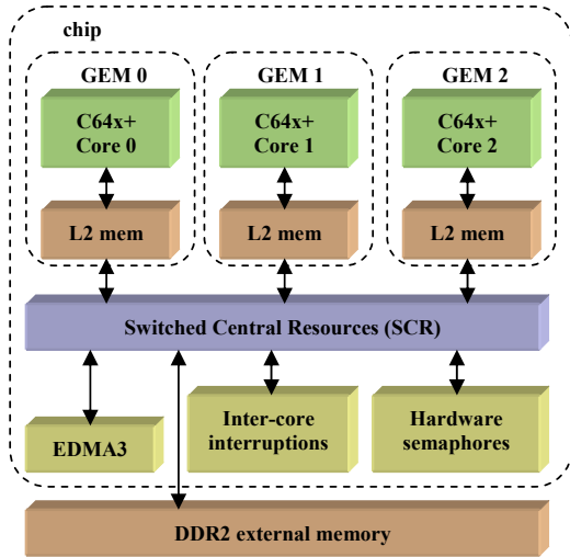
Fig. 19. TMS320TCI6487 architecture
