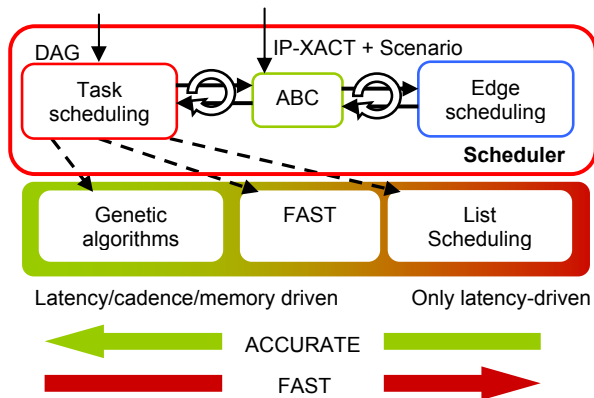
Fig. 10. Switchable scheduling heuristics
