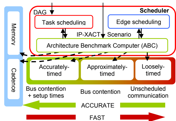
Fig. 11. Switchable ABC models
