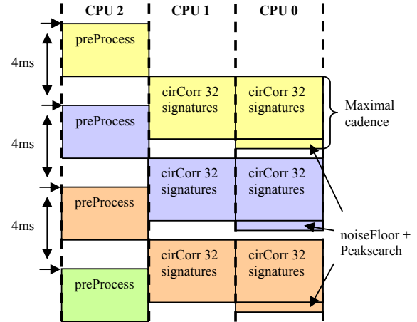
Fig. 20. Execution of the RACH-PD algorithm on a TMS320TCI6487
