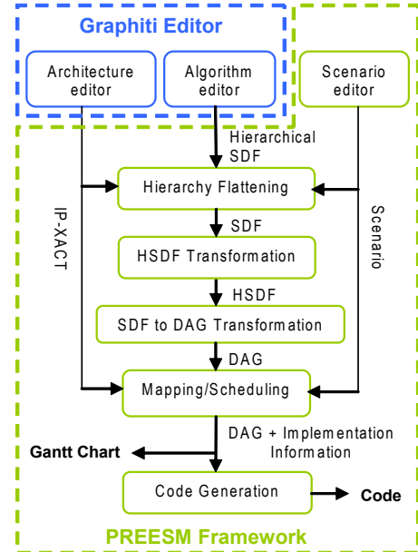
Fig. 8. Example of a workflow graph : From SDF and IP-XACT descriptions to the generated code
