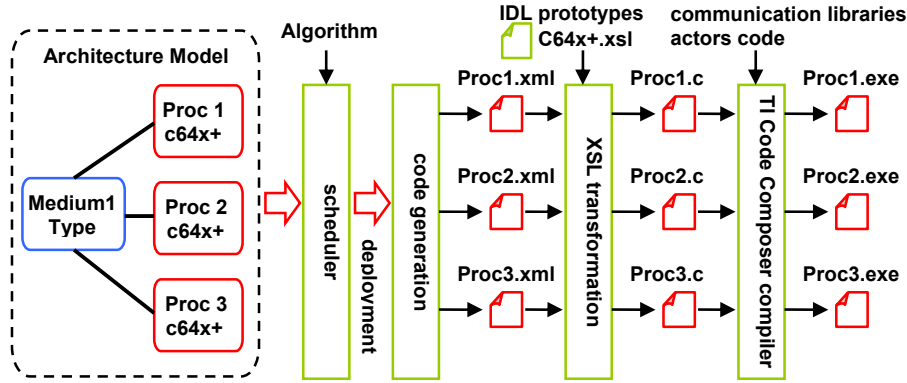
Fig. 12. Code generation
