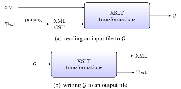
Fig. 2. Input/output with Graphiti's XML format \mathcal{G}
