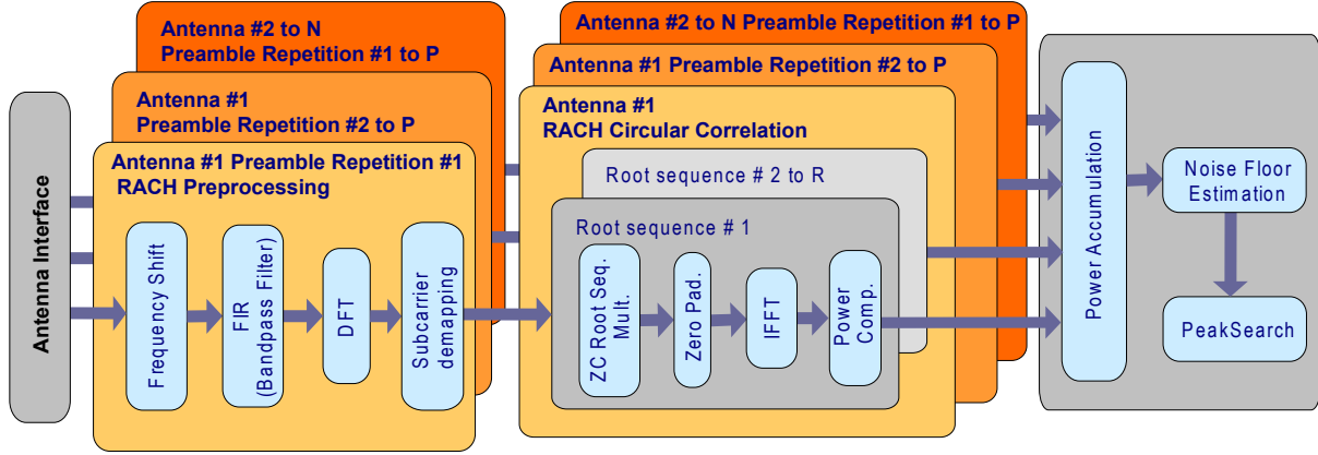
Fig. 16. Random Access Channel Preamble Detection (RACH-PD) Algorithm
