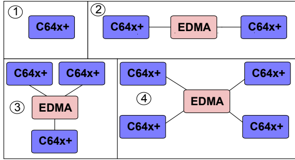
Fig. 17. Four architectures explored
