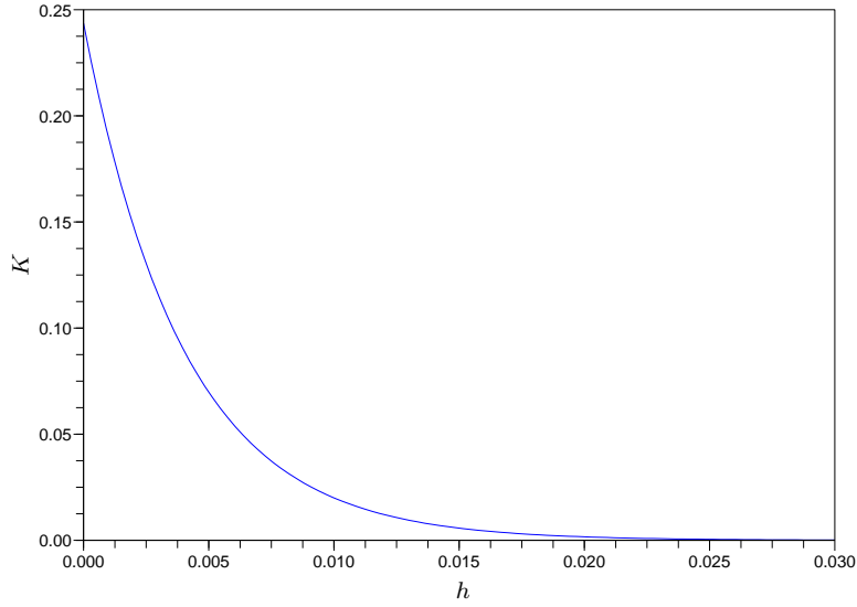
Figure 4: Shape of the friction term K(h) for \langle h_F \rangle = 0.01\text{ m}
