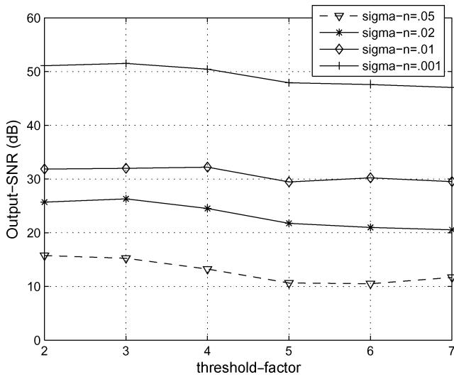
Fig. 8. Effect of the threshold in the IBA algorithm. The simulation parameters are m = 1024, n = 512, p = .9, \sigma_r = 1 and \mu = 10^{-7} . Results are averaged on 400 simulations.
