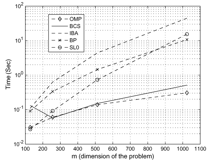
Fig. 10. Average CPU time in seconds versus problem dimension ( m ). For all dimensions n = 0.5m . The parameters are p = .9, \sigma_r = 1 and \sigma_n = .01 . The results are averaged on 400 simulations.
