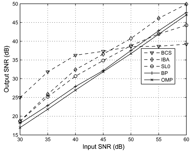
Fig. 5. Output-SNR versus Input-SNR. Results of the IBA algorithm compared with other algorithms. The simulation parameters are m = 1024, n = 512, p = .9, \sigma_r = 1, \alpha = .8 , and \mu = 10^{-7} . Five iterations are used for the M-step (steepest-ascent). Results are averaged on 400 simulations.
