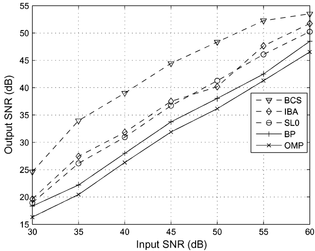
Fig. 6. Results of the IBA algorithm compared with other algorithms, for non BG sources. The simulation parameters are m = 1024 , n = 512 , p = .9 , \sigma_r = 1 , \alpha = .8 , and \mu = 10^{-7} . Five iterations are used for the M-step (steepest-ascent). Results are averaged on 400 simulations.
