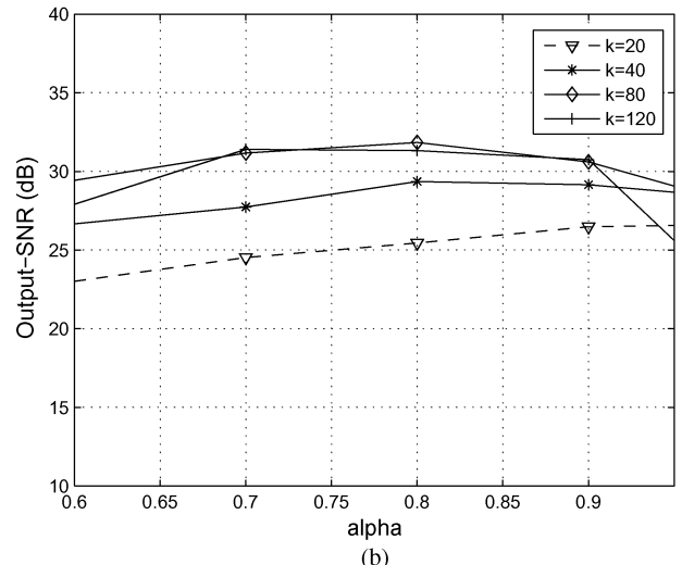
Fig. 7. Performance of the IBA algorithm versus parameter \alpha for m = 1024 , n = 512 and \sigma_r = 1 . In (a) k (number of active sources) is fixed to 100 and the effect of noise is investigated. In (b) \sigma_n is fixed to 0.01 and the effect of sparsity factor is analyzed. Values of k are 20, 40, 80, 120. Results are averaged on 400 simulations.
