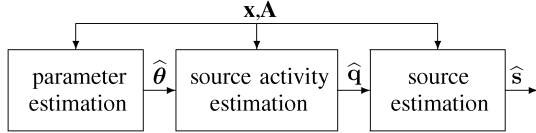
Fig. 1. Block diagram of our MAP algorithm.
