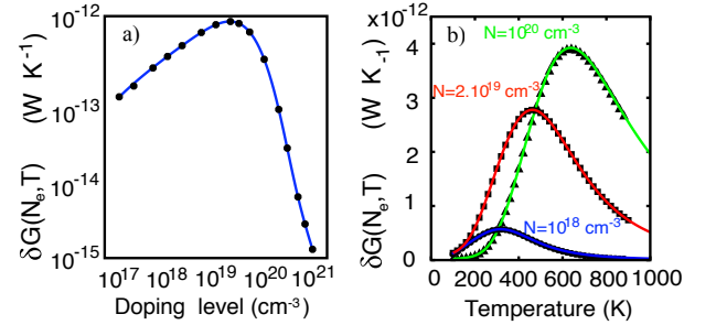
FIG. 3: Colors are available on-line. Comparison between the closed-form expression (plain line) of \delta G(N_e, T) and the exact numerical integration (symbols). a) Dependence on doping at T = 300 \text{ K} . b) Dependence on temperature for three doping concentrations.
