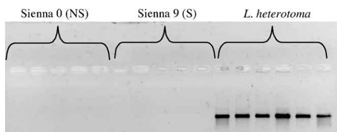
Fig. 1. Gel electrophoresis after PCR amplification using 16S generalist primers on non superparasitizing females L. boulandi (Sienna0), superparasitizing females L. boulandi (Sienna9) and females L. heterotoma naturally infected with the symbiotic bacteria Wolbachia .
