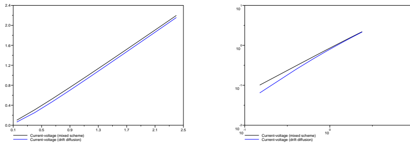
FIG. 5.1. Current-Voltage relation with doping 5 \times 10^{22} m^{-3} (left, normal scale; right, log scale).
