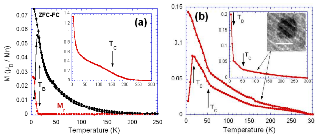
FIG. 2: Temperature dependence of magnetization in (a) Ga- \text{Ge}_{0.9}\text{Mn}_{0.1} and (b) As- \text{Ge}_{0.94}\text{Mn}_{0.06} : ZFC-FC curves at 0.015 T and magnetic remanence M_r after maximum field cooling at 5 T. Inset: in (a), saturation magnetization at 2 T, and in (b), TEM image of a \text{Ge}_3\text{Mn}_5 cluster.
