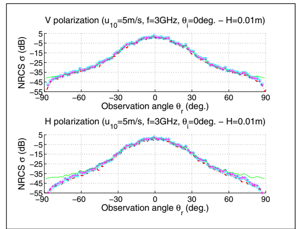
Figure 6. Bistatic NRCS of a contaminated sea for H = 10 mm: comparison between the reference numerical method and the KA+MSP, the SSA-1, and the WCA for both V and H polarizations, with and incidence angle \theta_i = 0 deg.
