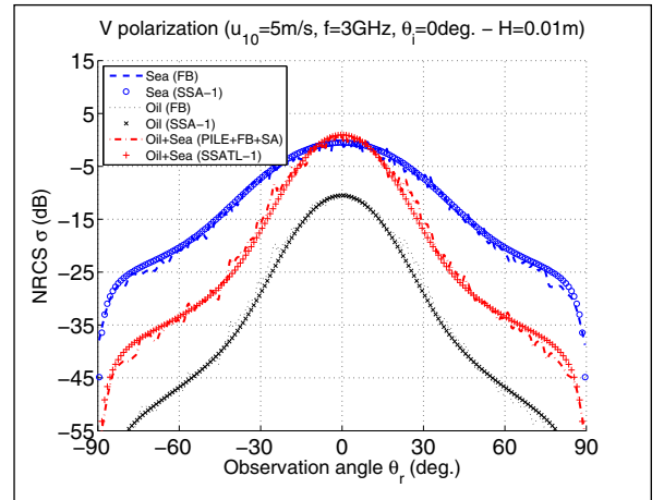
Figure 4. Bistatic scattering coefficients of clean and contaminated seas for V = 10 mm: comparison between the reference numerical method and the SSA-1. The wind speed is u_{10} = 5 m/s, the radar frequency f = 3 GHz, and the incidence angle \theta_i = 0 degrees.
