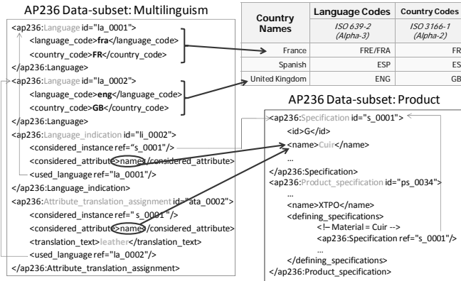
Fig. 10. AP236 Multilinguism Example
