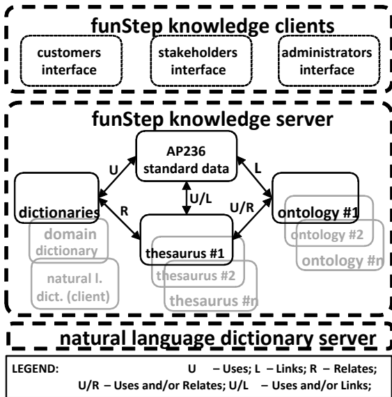
Fig. 7. funStep Knowledge Framework
