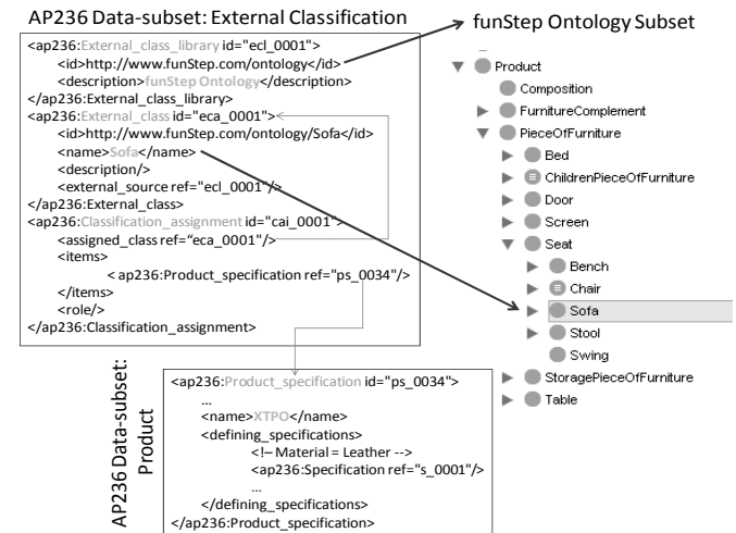
Fig. 9. AP236 External Classification Example
