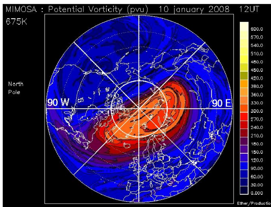
Fig. 2. Potential vorticity map calculated by the MIMOSA high-resolution advection model at 12:00 UT on 10 January 2008 at 675 K (about 27 km). The white circle at 72° N represents the geolocation of the tangent points of the GOMOS Sirius occultations in January 2008.
