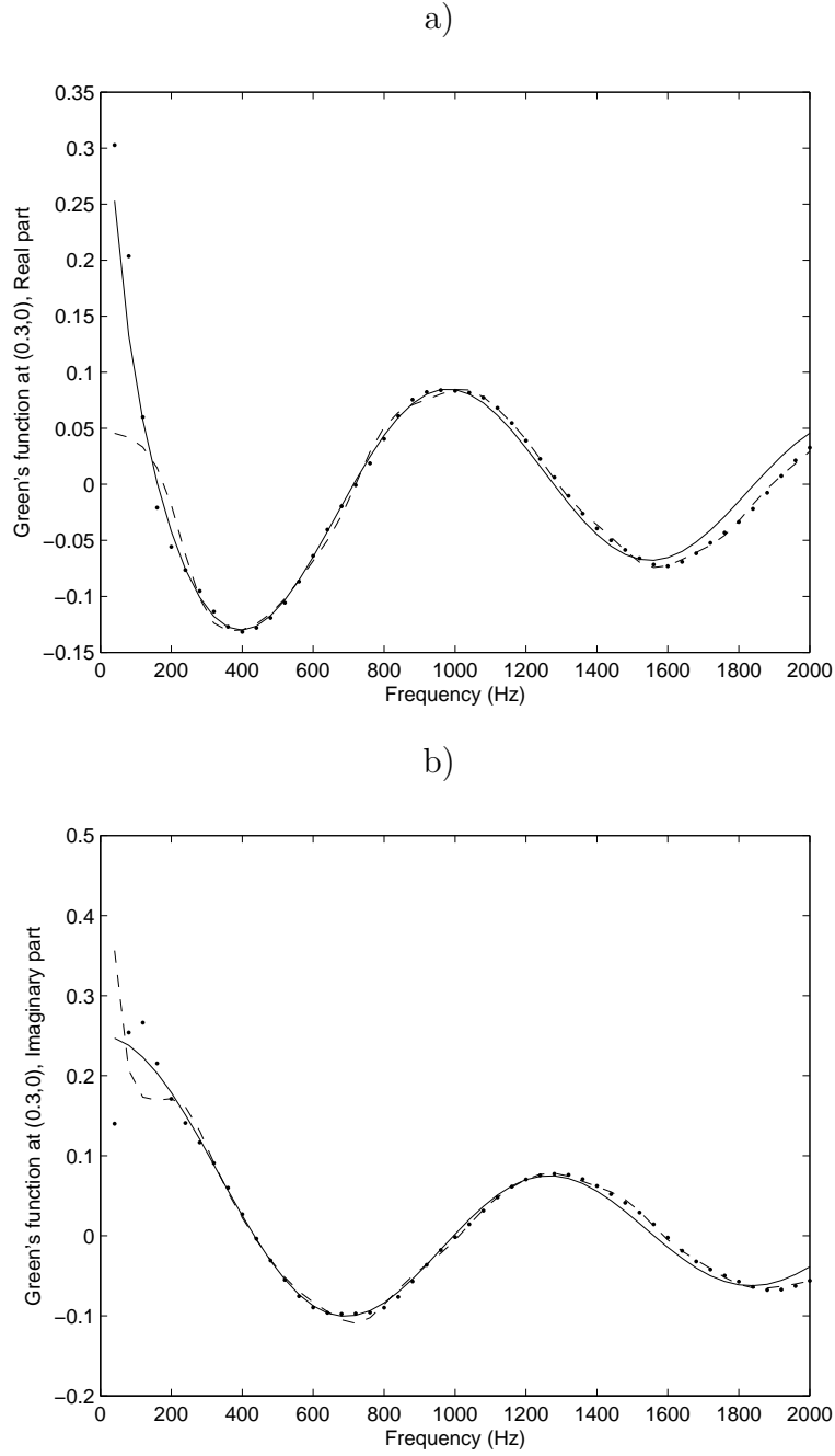
Fig. 10. Comparison of analytical — and numerical Green's functions, with the present method at order 0 -- and at order 2 . . for the 2D acoustics at point (0.3, 0) with L = 1m and b = 0.025m : a) real part, b) imaginary part.
