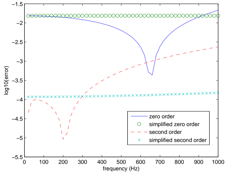
Fig. 6. Error versus the frequency for a plane wave at 10^\circ for (a) an element size 0.01m \times 0.01m and (b) an element size 0.05m \times 0.05m
