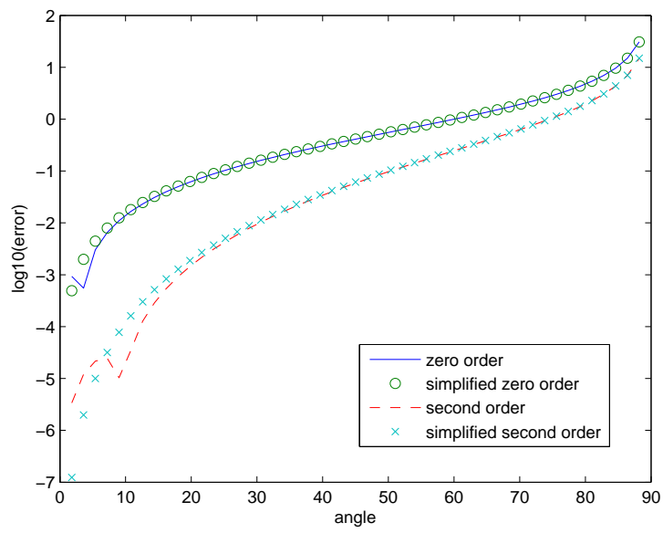
Fig. 7. Error versus the angle of incidence
