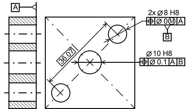
Figure 7: Tolerances of the experimental part.
