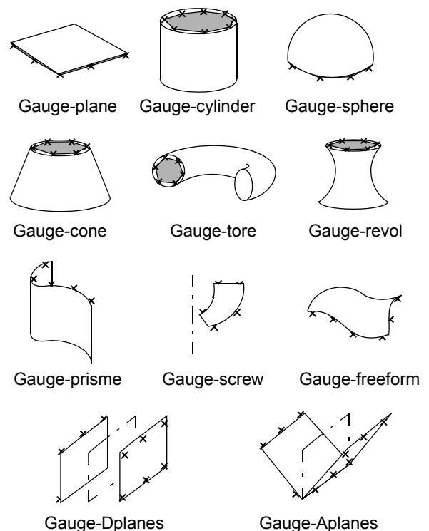
Figure 1: The Gauge-surfaces.
