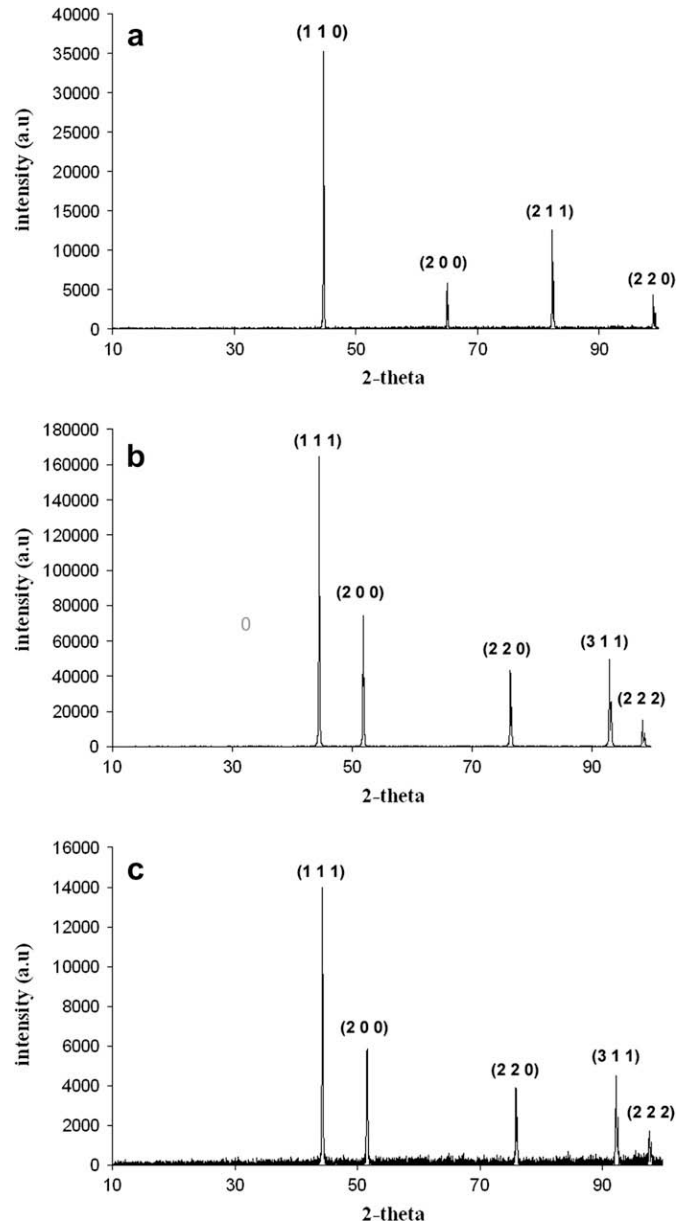
Fig. 4. X-ray diffraction patterns of iron powder reduced at 520 °C (a), nickel powder reduced at 410 °C (b) and cobalt powder reduced at 520 °C (c).
