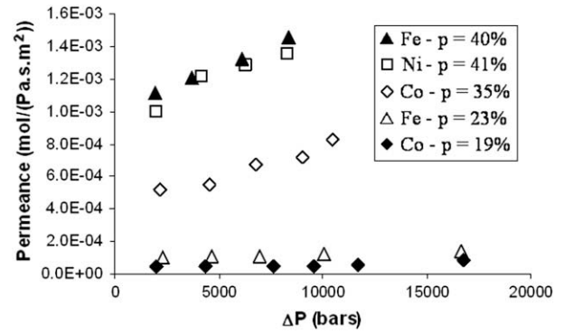
Fig. 11. Permeance behaviour of metal pellets with various porosities.
