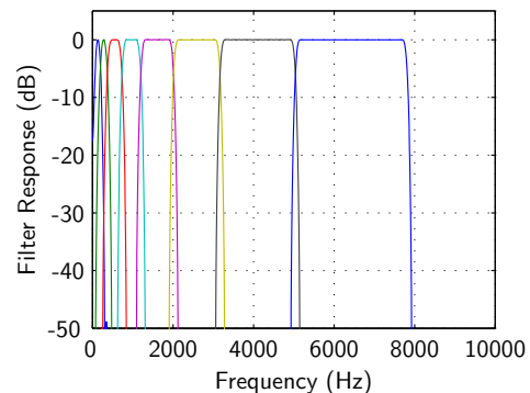
Figure 1: Graphical representation of the 8-channel filterbank response
