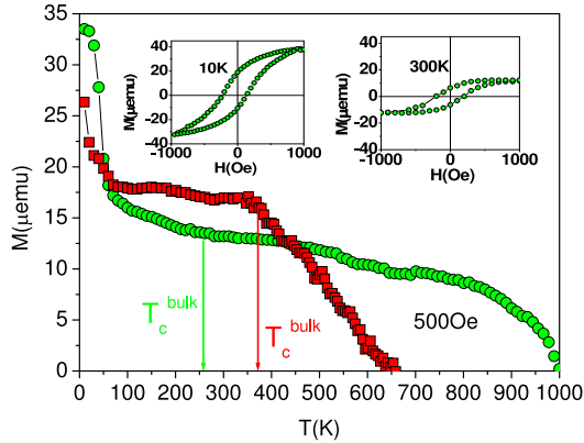
FIG. 4: (Color Online) Magnetization (500 Oersted) for the [(La_{2/3}Sr_{1/3}MnO_3)_3(BaTiO_3)_3]_{25} (red squares) and [(La_{2/3}Ca_{1/3}MnO_3)_4(BaTiO_3)_4]_{20} (green circles) superlattices. Hysteresis loops of the calcium super-lattice, recorded at 10 K and 300 K, are presented in the inserts. The arrows mark the bulk Curie temperatures. The surface of both samples is 16\text{mm}^2 .
