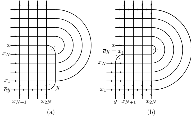
FIGURE 7. Proof of (31)
