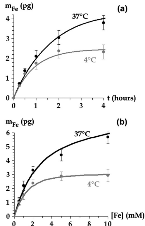
Fig. 3 Uptake curves for monocytes incubated at 4 °C and 37 °C, monitored as a function of the incubation time, t , ((a), [Fe] = 2 mM) or of the iron extracellular concentration [Fe] ((b), t = 2 h). Binding and incorporation with anionic magnetic nanoparticles were saturable with time and extracellular iron.
