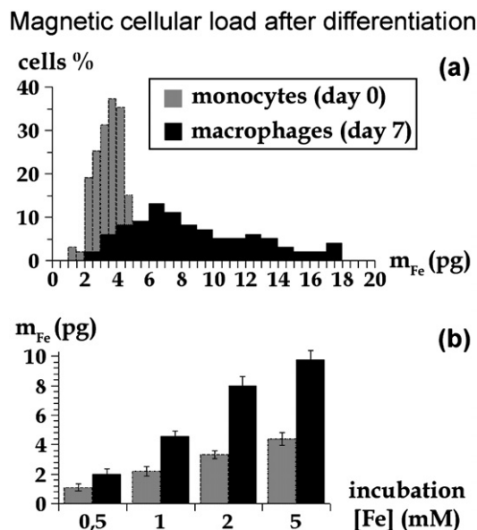
Fig. 6 Quantification of the iron load after the 6-day differentiation process. Monocytes were incubated for 2 h at 0.5, 1, 2 and 5 \text{mM}_{\text{Fe}} with corresponding iron load from 1.5 to 4 \text{pg}_{\text{Fe}} \text{ cell}^{-1} . For the 2 \text{mM}_{\text{Fe}} condition, distribution of the iron load is shown in (a). After the differentiation, the iron load is higher, in the range 2 to 10 \text{pg}_{\text{Fe}} \text{ cell}^{-1} for the four conditions (b), and much more distributed (a) with standard deviation in between 50 and 60%.
