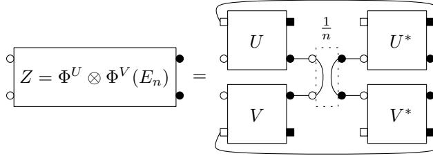
FIGURE 7. Z = \Phi^U \otimes \Phi^V(E_n)
