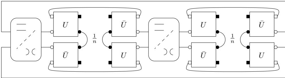
FIGURE 11. Developing \text{Tr}(n^2 Q Z Q)^2
