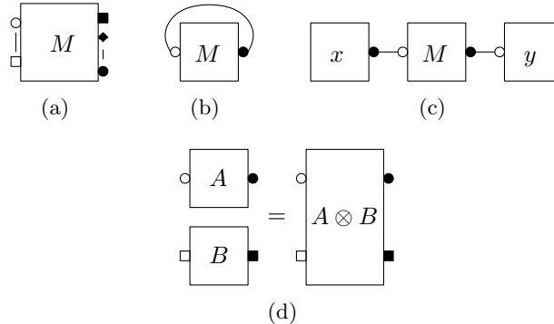
FIGURE 1. Basic diagrams and axioms
