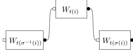
FIGURE 4. Monomials of traces of Wishart matrices
