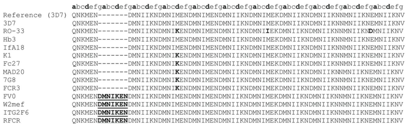
Figure 3. Alignment of P83 sequences amplified from 13 culture strains. SNP in P83 at nt position 863 T→A results in an amino acid change from Methionine (M) to a Lysine (K) at position 288 in PFC0345w gene product (red). This SNP was observed with a frequency of 0.38 (5/13). An insertion of DMNIKEN amino acid motif (bold and underlined) was detected with a frequency of 0.31 (4/13). doi:10.1371/journal.pone.0005419.g003
