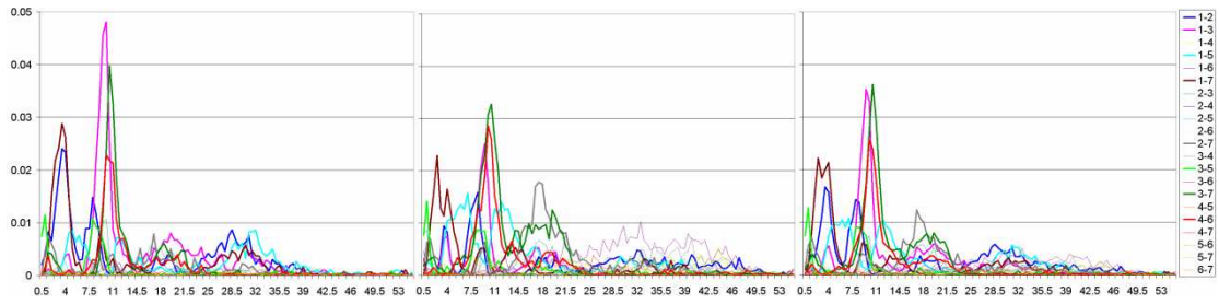
Figure 1. Lagged squared coherence ( S ) in the 0.5-55 Hz range (0.5 Hz resolution) for all pair-wise couples of the seven components of Fig. 2 for the BRL database (left), NTE database (center) and the combination of the two (right). The coherence profiles of significant ( p < 0.2 ) component pairs are drawn using a thick line.
