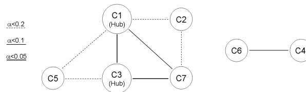
Figure 2. Significant lagged coherence ( S ) for three type II error rates ( \alpha ). Components with at least two significant connections at the 0.1 level and at least three significant connections at the 0.2 level are marked as “hubs”. The seven components organize in two fully independent networks.
