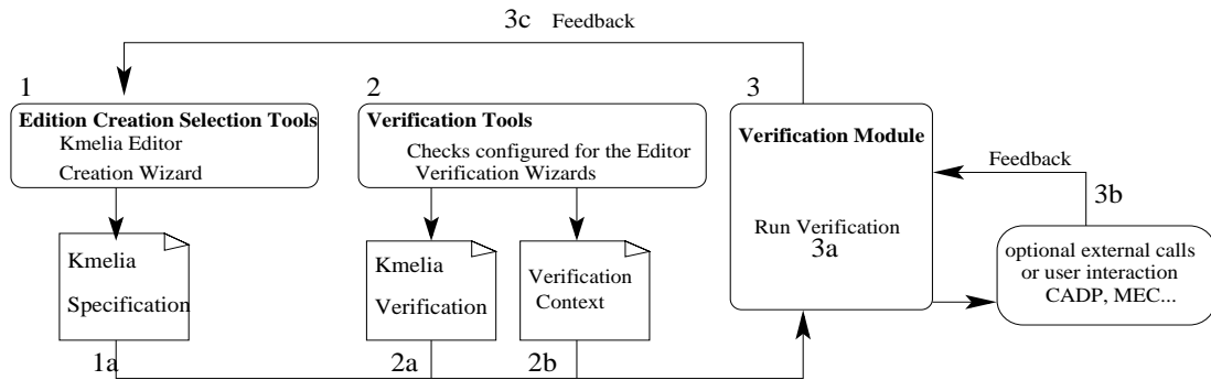
Fig. 2. Using Eclipse plugins to verify Kmelia components
