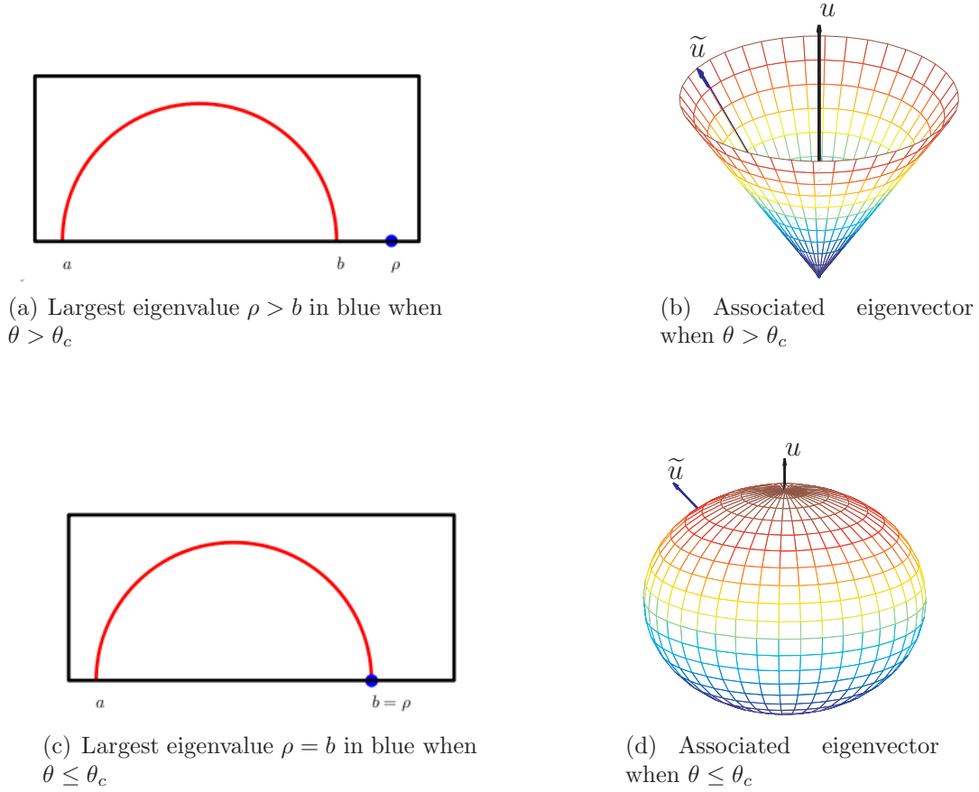
FIGURE 1. Assume that the limiting eigenvalue distribution of X_n is \mu_X with largest eigenvalue b . Consider the matrix P_n := \theta uu^* with rank r = 1 and largest eigenvalue \theta (> 0 , say). The vector u is an n \times 1 vector chosen uniformly at random from the unit n -sphere. The largest eigenvalue of X_n + P_n will differ from b if and only if \theta is greater than some critical value \theta_c . In this event, the largest eigenvalue will be concentrated around \rho with high probability as in (a). The associated eigenvector \tilde{u} will, with high probability, lie on a cone around u as in (b). When \theta \leq \theta_c , a phase transition occurs so that with high probability, the largest eigenvalue of the sum will equal b as in (c) and the corresponding eigenvector will be uniformly distributed on the unit sphere as in (d).
