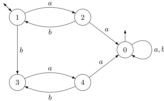
Figure 2. The minimal automaton of (ab)^* \cup A^*aaA^* .
