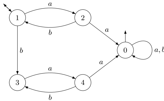
Figure 2. The minimal automaton of (ab)^* \cup A^*aaA^* .
