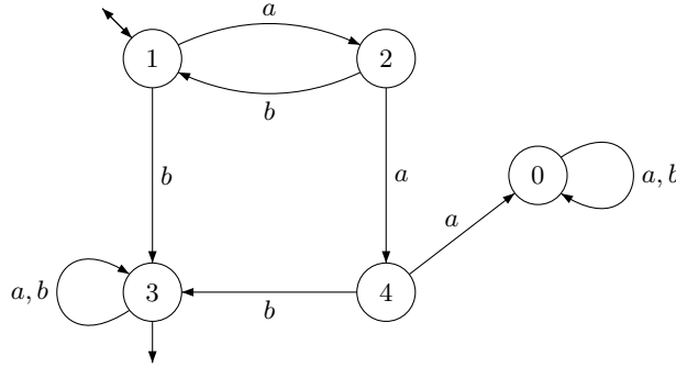
Figure 4. The minimal automaton of (ab)^* \cup (ab)^*bA^* \cup (ab)^*aabA^* .
