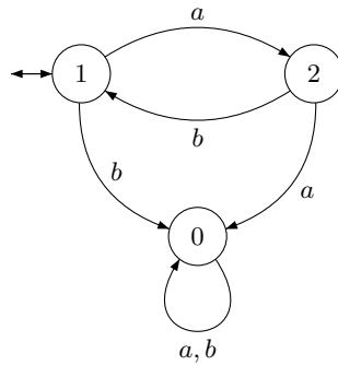
Figure 1. The minimal automaton of (ab)^* .
