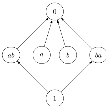
Figure 3. The order on B_2^{1-} .
