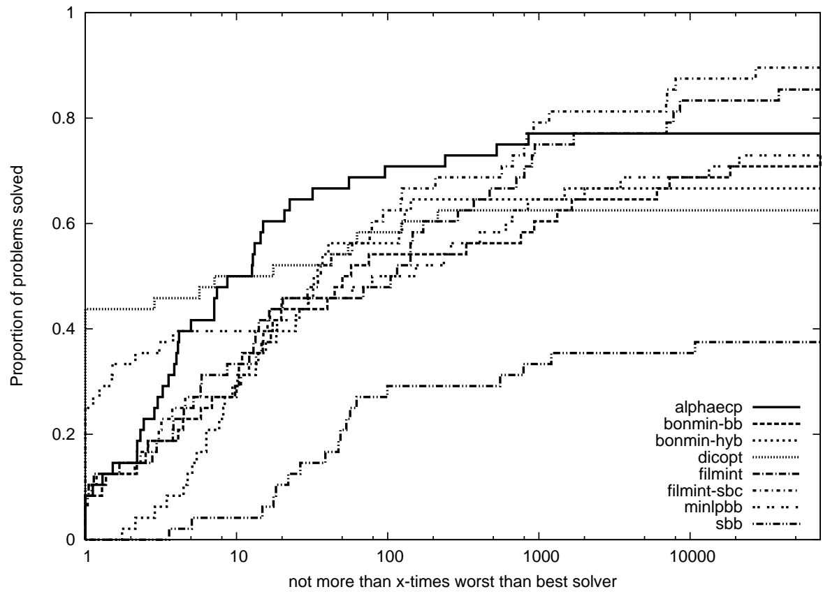
FIG. 1. Performance Profile Comparing Convex MINLP Solvers
