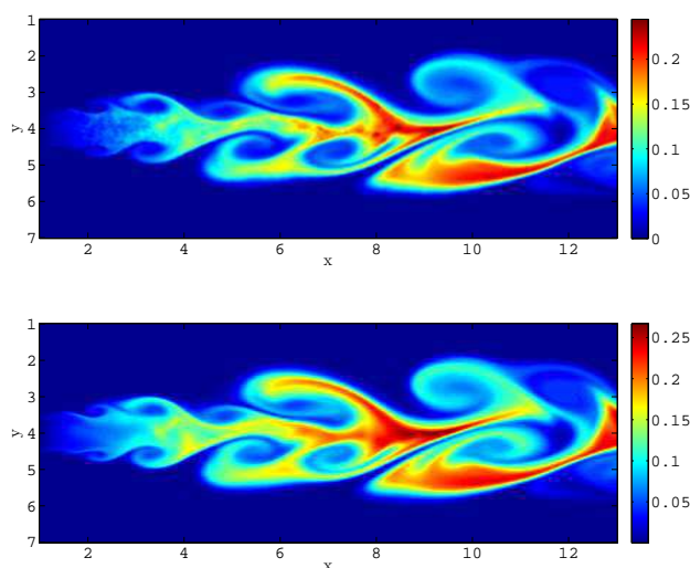
Figure 34: Comparison of the gaseous fuel mass fraction at time t = 20 , obtained from evaporation using (top) a Lagrangian method with 30,000 droplets at the considered time and (bottom) a Eulerian multi-fluid model with a 400 \times 200 \times 10 mesh.
