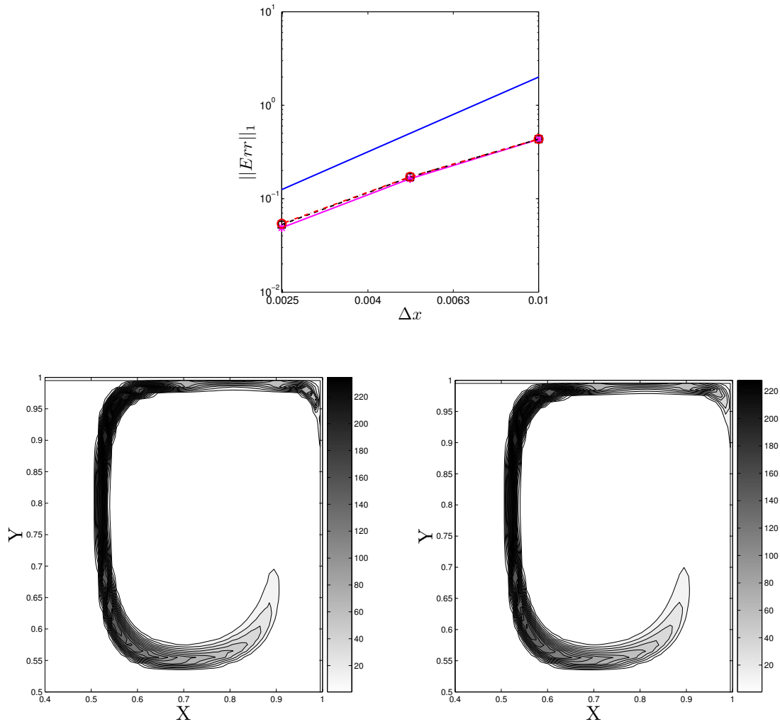
Figure 6: (top) Logarithm of L^1 norm of the error between Eulerian simulation for medium size droplets (fifth section St = 0.41 St_c ) for various \Delta x and the Lagrangian reference solution at time t = 1.5 , projected on the comparison grid 100 \times 100 \times 10 : slope two line (blue solid line), 10 sections (magenta solid line), 20 sections (dashed line) and 30 sections (dotted-dashed line). (bottom) Corresponding droplet mass density with 10 iso-contours from 0 up to 1.44-time the maximum of the initial mass density in the fifth section : (left) Lagrangian reference solution, (right) Eulerian computation with a 400 \times 400 \times 10 grid.
