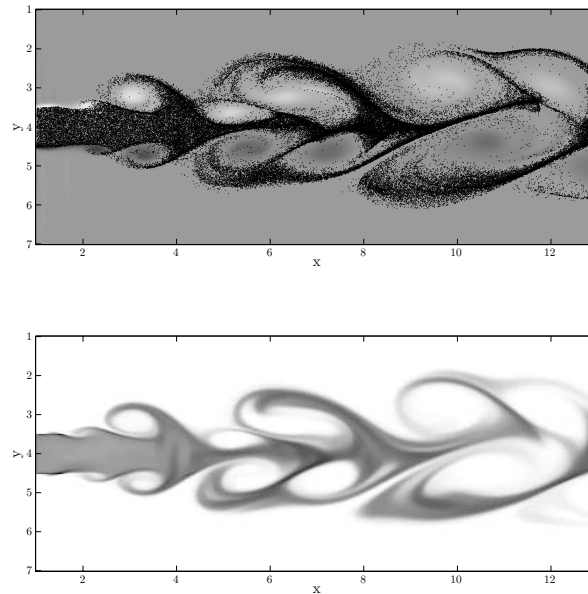
Figure 30: Non-evaporating polydisperse spray, Stokes 0.011 to 1.1 corresponding to diameters d = 9 \mu m to d = 90 \mu m , at time t=20 , : (top) Lagrangian particle positions with 70000 particles, (bottom) Eulerian total number density with a 400 \times 200 \times 5 grid.
