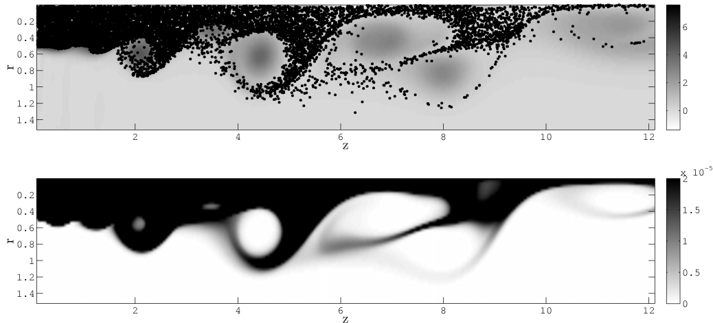
Figure 14: Evaporating polydisperse spray , Stokes 0.003 to 4.45 corresponding to diameters d = 4 \mu m to d = 150 \mu m , at time t=15 , : (top) Lagrangian particle positions with 10000 particles, (bottom) Eulerian total number density with a 400 \times 200 \times 5 grid.
