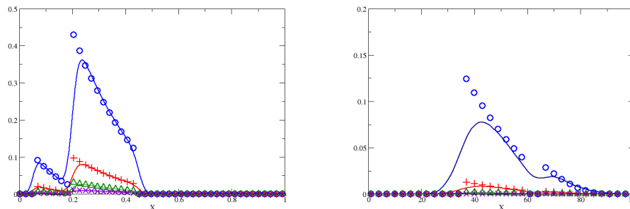
Figure 22: Numerical moments (solid lines from top- 0^{th} order moment down to bottom- 3^{rd} order moment) computed with high order moment method for size and high order moment method for velocity, compared with the analytical moments (circles : zeroth order moment, vertical crosses : first order moment, triangles : second order moment, diagonal crosses : third order moment), at two instants : t = 0.4 (left) and t = 0.7 (right)
