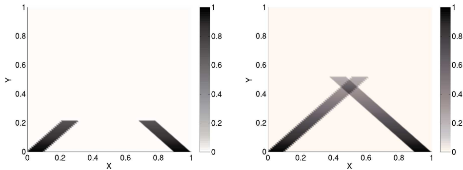
Figure 23: Total droplet number density of evaporating jets crossing simulated with high order moment methods for size and velocity, at two instants : t = 0.2 (left) and t = 0.5 (right), on a 100 \times 100 grid
