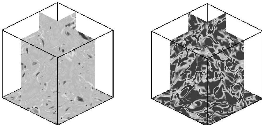
Figure 39: Eulerian spray number density in perpendicular planes inside the domain, obtained with the multi-fluid method on a 129^3 Cartesian grid : (left) St = 0.17 , (right) St = 1.05 .
