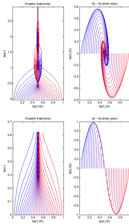
Figure 1: (top) : St = 0.3 , St > St_c , characteristic crossing in the (x, t) plane (left) and phase plane dynamics (x, v) (right) for 30 initial conditions equally distributed in space with zero initial velocity; (bottom) : St = 0.03 , St < St_c , no characteristic crossing in the (x, t) plane (left) and phase plane dynamics (x, v) (right) for 30 initial conditions equally distributed in space with zero initial velocity.
