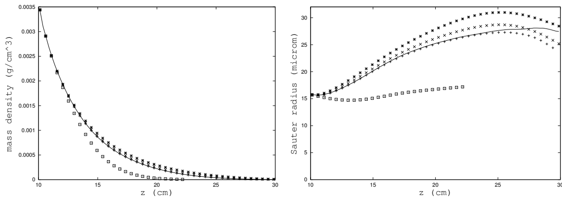
Figure 18: (left) Evolution of the mass density of liquid for the Lagrangian reference solution (solid line) and for various discretizations with the Eulerian multi-fluid model ( + : 90 sections, × : 30 section, * : 15 sections, □ : 90 sections without collision). (right) Sauter mean radius for the Lagrangian reference solution (solid line) and for various discretizations with the Eulerian multi-fluid model ( + : 90 sections, × : 30 section, * : 15 sections, □ : 90 sections without collision).
