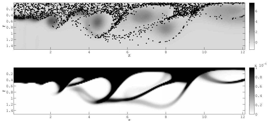
Figure 13: Non-evaporating polydisperse spray, high inertia droplets , Stokes 0.71 to 4.45 corresponding to diameters d = 60 \mu m to d = 150 \mu m , at time t=15 : (top) Lagrangian particle positions with 40000 particles, (bottom) Eulerian total number density with a 400 \times 200 \times 5 grid.
