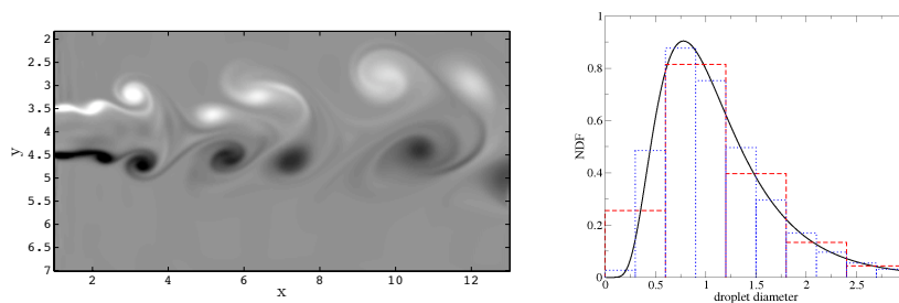
Figure 29: Free jet configuration: (left) gaseous vorticity at time t=20 , obtained on a 400 \times 200 grid; (right) polydisperse log-normal distribution discretized with 5 (dashed lines) to 10 (dotted lines) sections.
