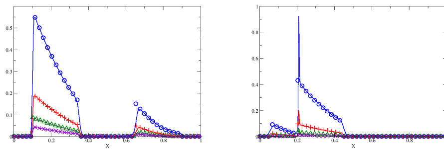
Figure 21: Numerical moments (solid lines from top- 0^{th} order moment down to bottom- 3^{rd} order moment) computed with high order moment method for size but pressureless gas dynamics for the velocity modeling, compared with the analytical moments (circles : zeroth order moment, vertical crosses : first order moment, triangles : second order moment, diagonal crosses : third order moment), at two instants : t = 0.2 (left) and t = 0.4 (right)
