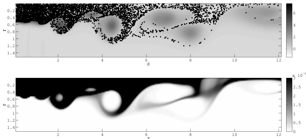
Figure 15: Evaporating polydisperse spray, low inertia droplets , Stokes 0.003 to 0.18 corresponding to diameters d = 4 \mu m to d = 30 \mu m , at time t=15 : (top) Lagrangian particle positions with 10000 particles, (bottom) Eulerian number density with a 400 \times 200 \times 5 grid.
