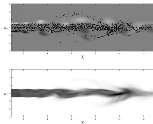
Figure 37: Evaporating polydisperse spray, high inertia droplets, Stokes from 0.48 to 1.1 corresponding to diameters d = 60 \mu\text{m} to d = 90 \mu\text{m} , at time t=15 : (top) Lagrangian particle positions with 7,000 particles over gas vorticity, (bottom) Eulerian number density with a 400 \times 200 \times 10 grid.
