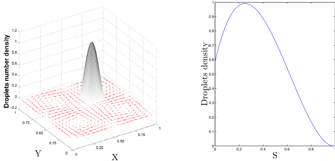
Figure 3: Initial droplet distribution : (left) non uniform spatial repartition, three-dimensional plot with number density as the third coordinate; (right) non-dimensional polydisperse size distribution.
