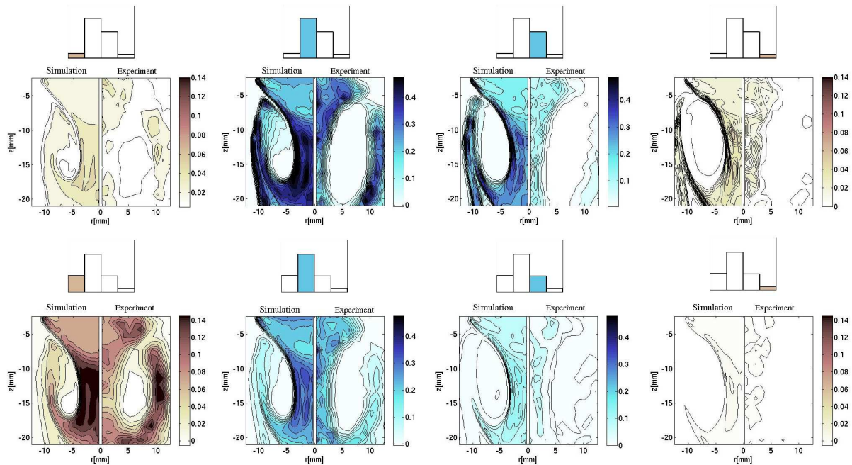
Figure 28: Comparison of size-conditioned decane (top) and methanol (bottom) droplet number density (droplet/mm 3 ) between 120 phase-locked IPI experimental measurements with a reduced field of view of 27×20 mm 2 (right half) and numerical simulations on a 400 × 400 grid (left half) at phase \pi . Four size ranges are presented from left to right, range [6,15] [15,30] [30,45] [45,60] in \mu\text{m} . Small histograms represent the droplet number repartition among the four size ranges. Two scales are used. Very small and big droplets have low concentration level and are presented in ochre, whereas the high concentration levels of droplets of inter size are presented in blue.
