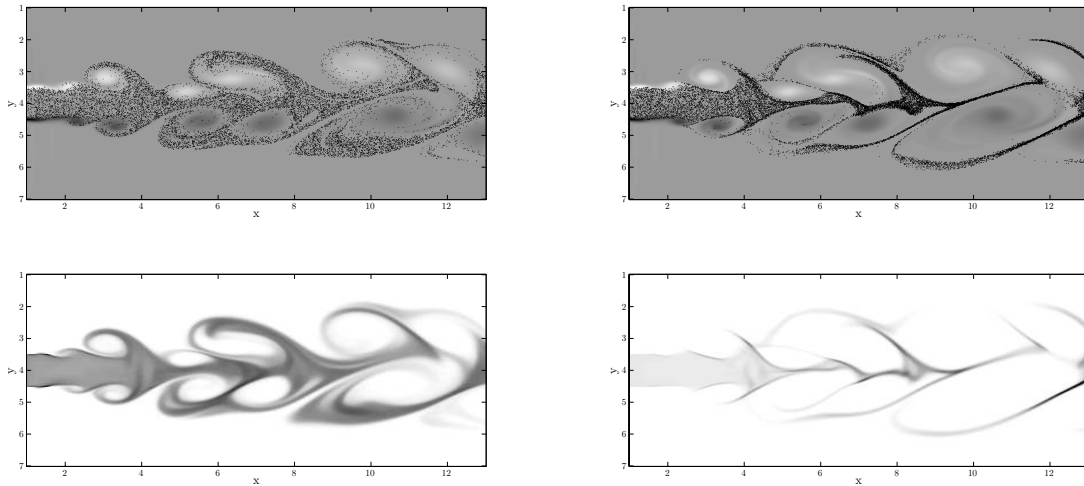
Figure 31: Non-evaporating polydisperse spray at time t=20 : (left) low inertia droplets, Stokes 0.011 to 0.12 corresponding to diameters d = 9 \mu\text{m} to d = 30 \mu\text{m} , (right) high inertia droplets, Stokes 0.48 to 1.1 corresponding to diameters d = 60 \mu\text{m} to d = 90 \mu\text{m} ; (top) Lagrangian particle positions with 40,000 particles over gas vorticity, (bottom) Eulerian number density on a 400 \times 200 \times 5 grid.
