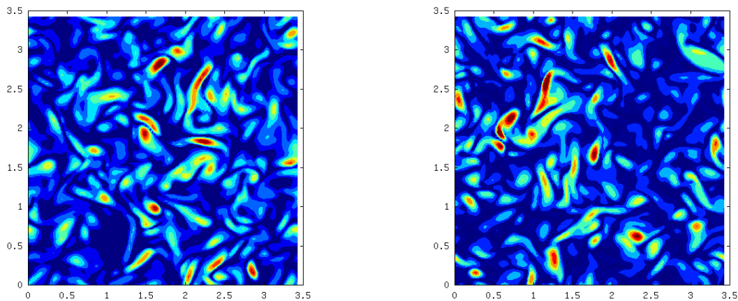
Figure 40: Gas vorticity square norm in the (y - z) plane at x = 1.75 and in the (x - y) plane at z = 1.75 .
