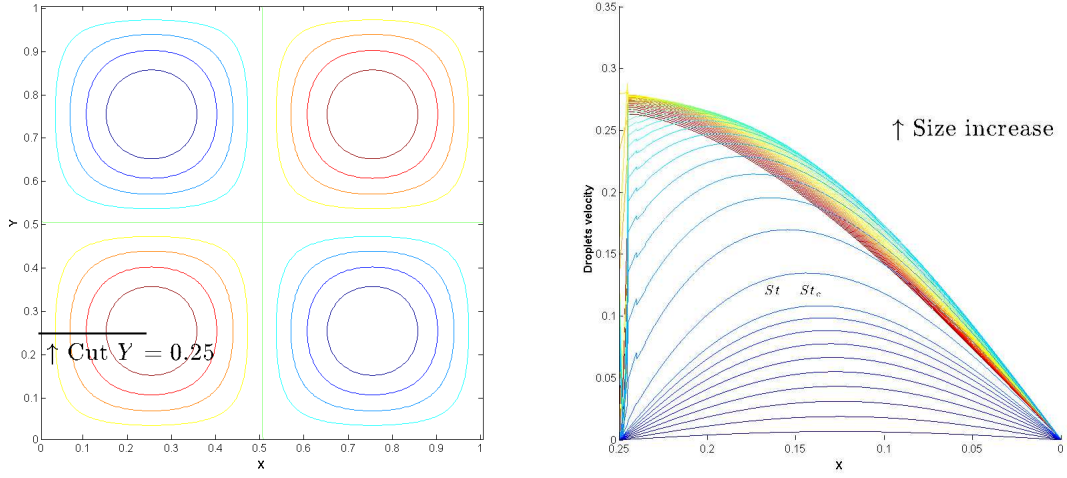
Figure 2: (left) Stream lines of the Taylor-Green vortices and position of the cut for the study of normal ejection velocity, (right) Structure of the invariant droplet velocity manifold versus Stokes number in term of the velocity component orthogonal to the gas flow.
