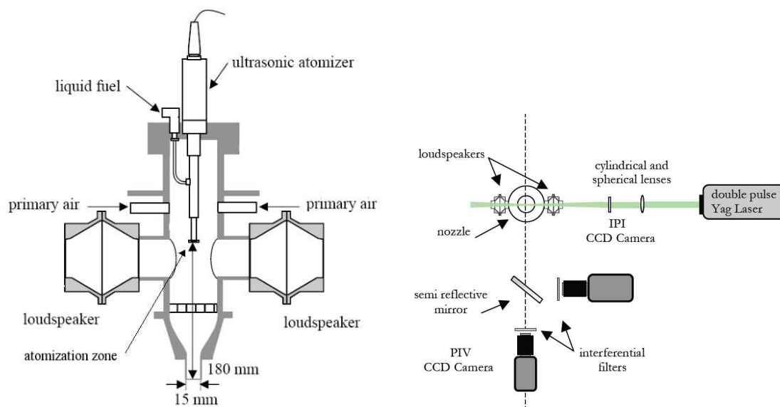
Figure 25: (left) Lateral view of the experimental setup, (right) PIV and IPI experimental set-up.
