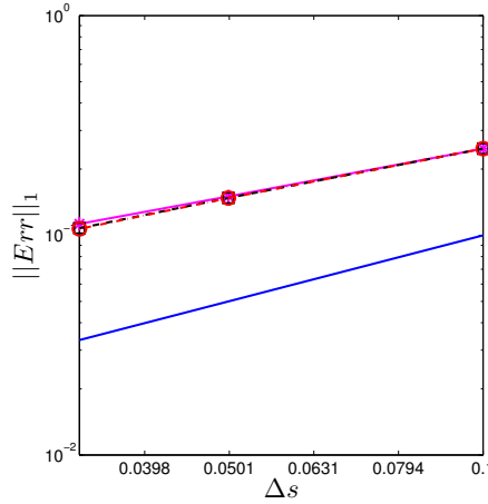
Figure 9: Logarithm of L^1 norm of the error between Eulerian simulation for inertial droplets (ninth section St = 0.78 St_c ) for various \Delta S at fixed \Delta x and the Lagrangian reference solution at time t = 1.5 projected on the comparison grid 100 \times 100 \times 10 in the evaporating case : slope one line (blue solid line), \Delta x = 1/100 (magenta solid line), \Delta x = 1/200 (dashed line) and \Delta x = 1/400 (dotted-dashed line).
