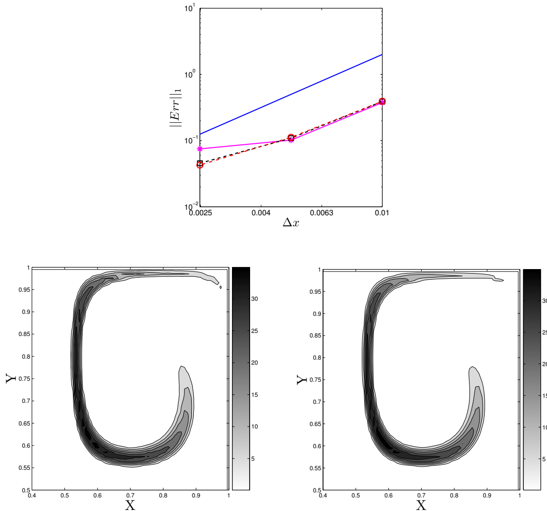
Figure 5: (top) Logarithm of L^1 norm of the error between Eulerian simulation for small droplets (second section St = 0.14 St_c ) for various \Delta x and the Lagrangian reference solution at time t = 1.5 , projected on the comparison grid 100 \times 100 \times 10 : slope two line (blue solid line), 10 sections (magenta solid line), 20 sections (dashed line) and 30 sections (dotted-dashed line). (bottom) Corresponding droplet mass density with 10 iso-contours from 0 up to 1.44-time the maximum of the initial mass density in the second section : (left) Lagrangian reference solution, (right) Eulerian computation with a 400 \times 400 \times 10 grid.
