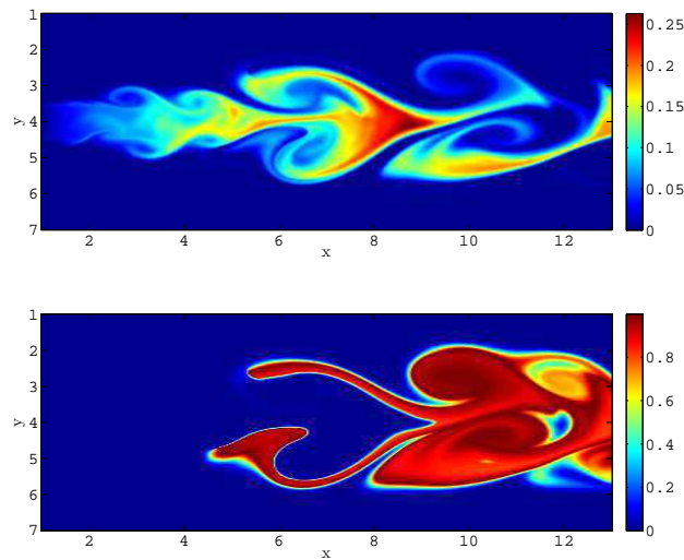
Figure 35: Coldflame at time t=20 using a Eulerian multi-fluid model with a 400 \times 200 \times 10 mesh : (top) gaseous fuel mass fraction; (bottom) burnt gas mass fraction.
