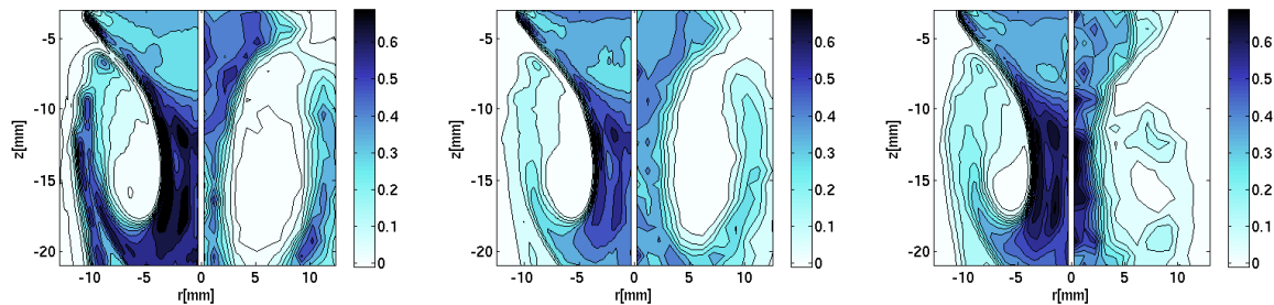
Figure 27: Comparison between IPI experimental measurements - averaged field obtained from 120 instantaneous phase-locked samples with a reduced field of view of 27 \times 20 \text{ mm}^2 (right half) and numerical simulations on a 400 \times 400 grid (left half): total droplet concentration at phase \pi in droplet/ \text{mm}^3 ; from left to right: decane (non evaporating reference liquid), methanol and heptane (evaporating liquids).
