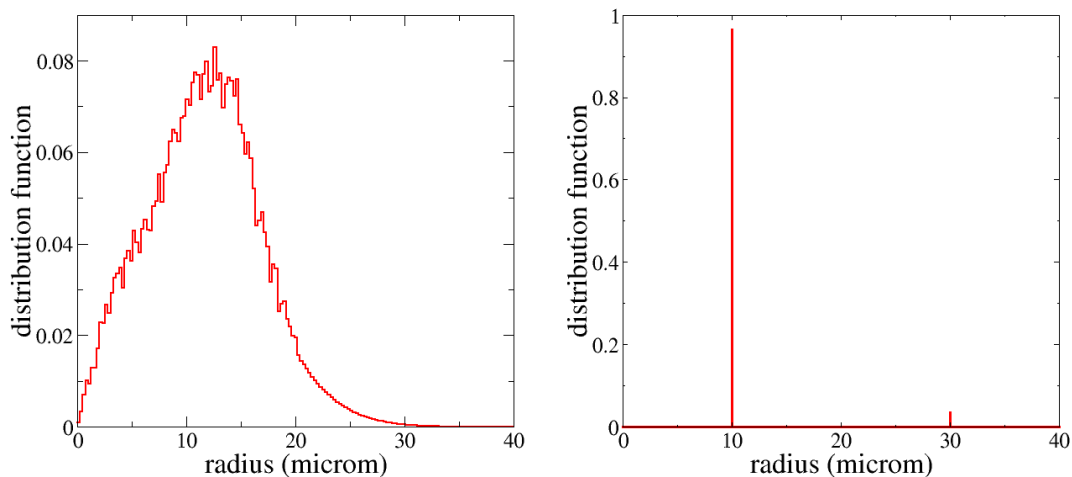
Figure 17: (left) Monomodal distribution function from experimental measurements, (right) Bimodal distribution function.
