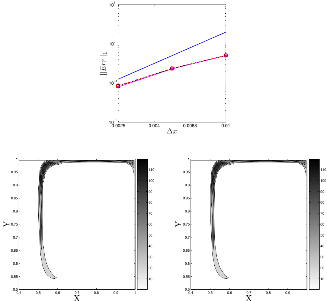
Figure 7: (top) Logarithm of L^1 norm of the error between Eulerian simulation for inertial droplets (ninth section St = 0.78 St_c ) for various \Delta x and the Lagrangian reference solution at time t = 1.5 , projected on the comparison grid 100 \times 100 \times 10 : slope two line (blue solid line), 10 sections (magenta solid line), 20 sections (dashed line) and 30 sections (dotted-dashed line). (bottom) Corresponding droplet mass density with 10 iso-contours from 0 up to 2.43-time the maximum of the initial mass density in the ninth section : (left) Lagrangian reference solution, (right) Eulerian computation with a 400 \times 400 \times 10 grid.
