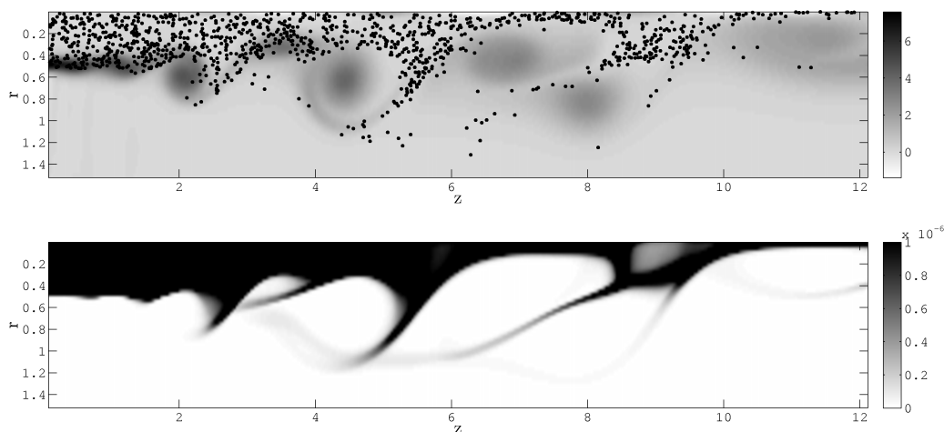
Figure 16: Evaporating polydisperse spray, high inertia droplets , Stokes 0.71 to 4.45 corresponding to diameters d = 60 \mu m to d = 150 \mu m , at time t=15 : (top) Lagrangian particle positions with 10000 particles, (bottom) Eulerian total number density with a 400 \times 200 \times 5 grid.
