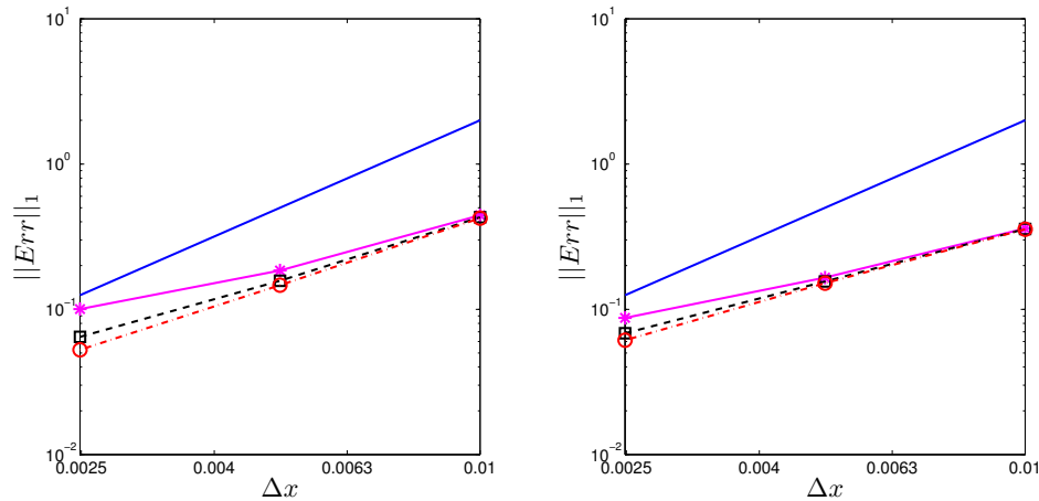
Figure 8: Logarithm of L^1 norm of the error between Eulerian simulation (left) for small droplets (second section St = 0.14 St_c ), (right) for medium size droplets (fifth section St = 0.41 St_c ) for various \Delta x and the Lagrangian reference solution at time t = 1.5 , projected on the comparison grid 100 \times 100 \times 10 in the evaporating case : slope two line (blue solid line), 10 sections (magenta solid line), 20 sections (dashed line) and 30 sections (dotted-dashed line).
