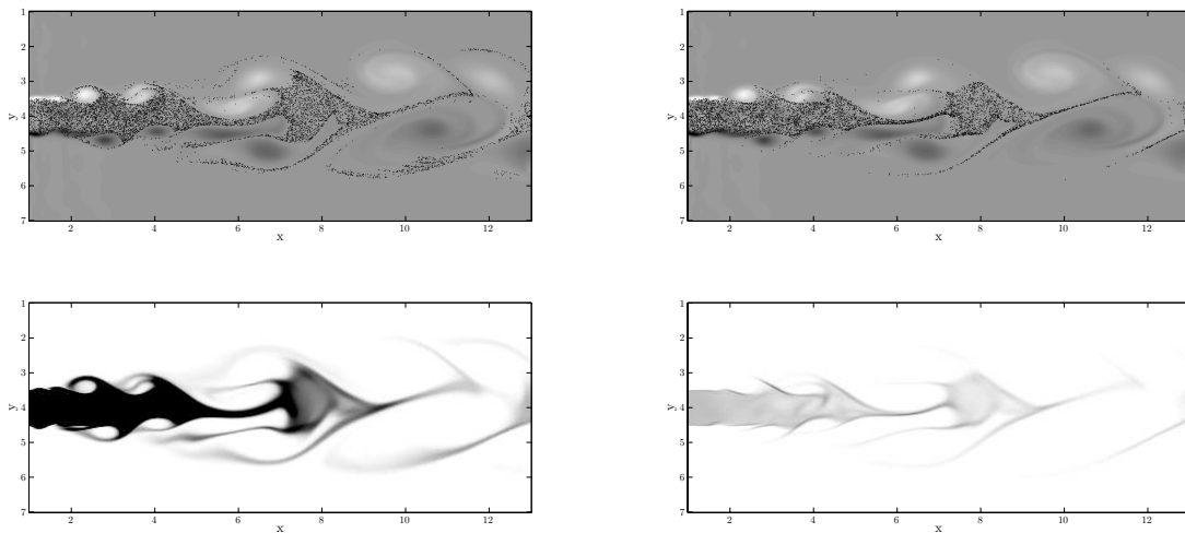
Figure 33: Evaporating polydisperse spray at time t=20 : (left) low inertia droplets, Stokes 0.011 to 0.12 corresponding to diameters d = 9 \mu\text{m} to d = 30 \mu\text{m} , (right) high inertia droplets, Stokes 0.48 to 1.1 corresponding to diameters d = 60 \mu\text{m} to d = 90 \mu\text{m} ; (top) Lagrangian particle positions with 7,000 particles over gas vorticity, (bottom) Eulerian number density with a 400 \times 200 \times 10 grid.
