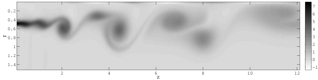
Figure 10: Gaseous vorticity at time t=15 , obtained with a low mach number dilatible solver on a 400 \times 200 grid.
