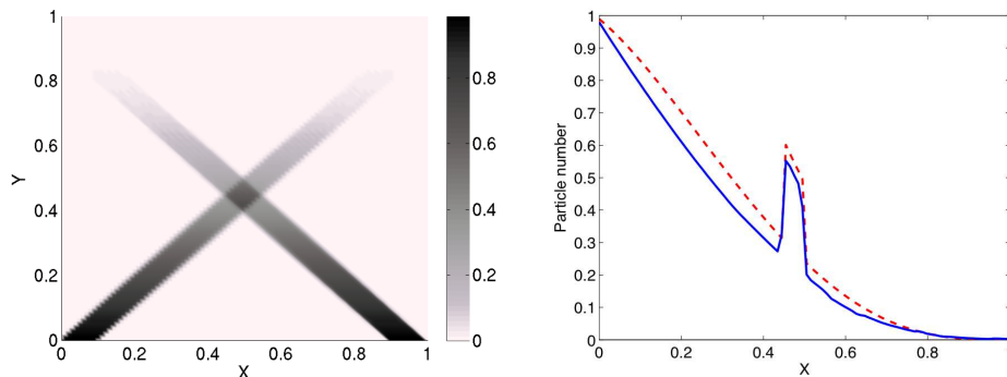
Figure 24: Total droplet number density of evaporating jets crossing simulated with high order moment methods for size and velocity at t = 1 on a 100 \times 100 grid (left) and comparison of the number density of the numerical solution (solid line) and the analytical solution (dashed line).
