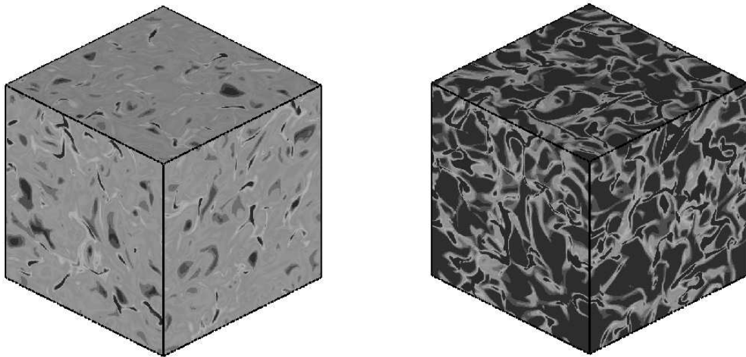
Figure 38: Eulerian spray number density at the edges of the domain, obtained with the multi-fluid method on a 129^3 Cartesian grid : (left) St = 0.17 , (right) St = 1.05 .
