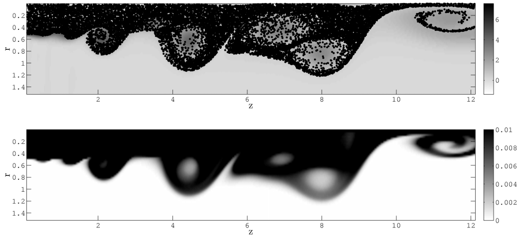
Figure 12: Non-evaporating polydisperse spray, low inertia droplets , Stokes 0.003 to 0.18 corresponding to diameters d = 4 \mu m to d = 30 \mu m , at time t=15 : (top) Lagrangian particle positions with 40000 particles, (bottom) Eulerian number density with a 400 \times 200 \times 5 grid.
