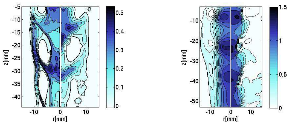
Figure 26: Comparison between experimental measurements - averaged field obtained from 20 instantaneous phase-locked samples (right half) for a 59 \times 44 \text{ mm}^2 field of view and numerical simulations on a 400 \times 400 grid (left half): decane droplet concentration (droplet/ \text{mm}^3 - left) and mean droplet axial velocities ( \text{m.s}^{-1} - right) for the phase \phi = 0 (arbitrary reference).
