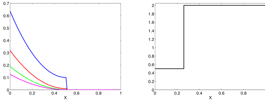
Figure 20: (left) Initial condition for the moments (the highest curve describes the 0^{th} order moment down to the lowest curve which corresponds to the 3^{rd} order moment, (right) Initial condition for the velocity field of the droplets.
