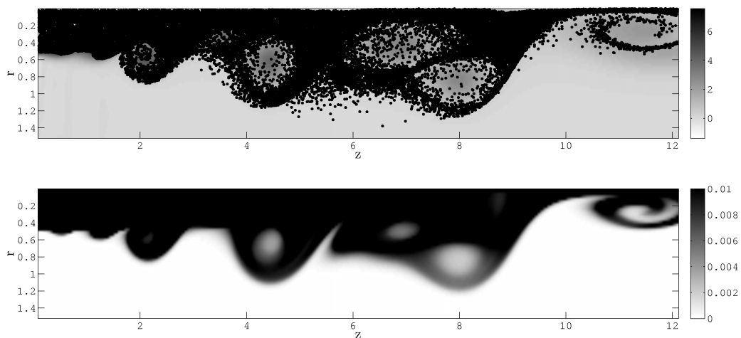
Figure 11: Non-evaporating polydisperse spray , Stokes 0.003 to 4.45 corresponding to diameters d = 4 \mu m to d = 150 \mu m , at time t=15 , : (top) Lagrangian particle positions with 40000 particles, (bottom) Eulerian total number density with a 400 \times 200 \times 5 grid.
