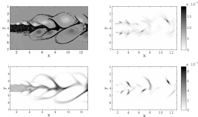
Figure 36: Non-evaporating polydisperse spray, high inertia droplets, Stokes from 0.48 to 1.1 corresponding to diameters d = 60 \mu\text{m} to d = 90 \mu\text{m} , at time t=20 : (left-top) Lagrangian particle positions with 20,000 particles over gas vorticity, (left-bottom) Eulerian number density with a 400 \times 200 \times 5 grid. Evaluation of the trace of the covariance matrix (right-top) as well as the absolute value of the difference between the two eigenvalues highlighting the zones of droplet crossing (right-bottom).
