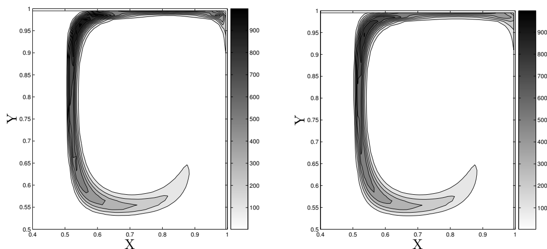
Figure 4: Zoom on the top-right quarter of the periodic computational domain of the total mass density of droplets at time t = 1.5 , projected on the comparison grid 100 \times 100 \times 10 : (left) Lagrangian reference solution, (right) Eulerian with a 400 \times 400 \times 10 grid.
