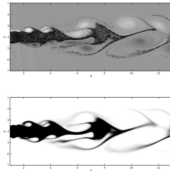
Figure 32: Evaporating polydisperse spray, Stokes 0.011 to 1.1 corresponding to diameters d = 9 \mu\text{m} to d = 90 \mu\text{m} , at time t=20 , : (top) Lagrangian particle positions with 30,000 particles, (bottom) Eulerian total number density with a 400 \times 200 \times 5 grid.
